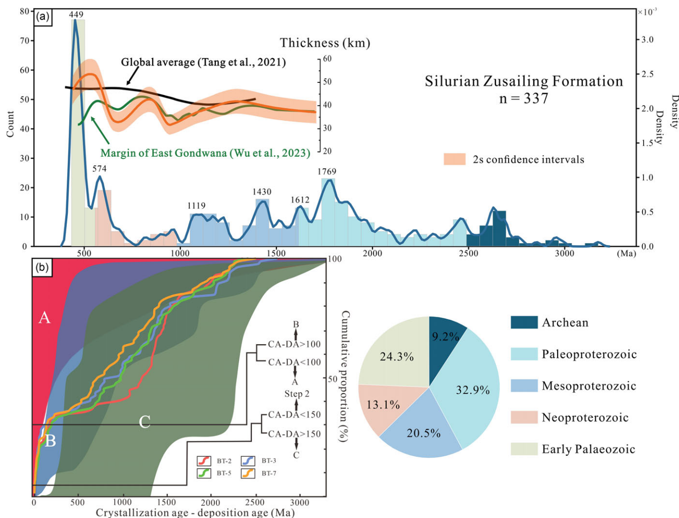
Figure 6. (Colour online) (a) Kernel density estimate (KDE) diagrams of detrital zircon U–Pb ages from Zusailing Formation and Crustal thickness between 435–1800 Ma modelled by zircon anomalies \text{Eu}/\text{Eu}^* (chondrite-normalized \text{Eu}/\sqrt{\text{Sm} \times \text{Gd}} ). The black and green curves represent global compilation (Tang et al. 2021) and the margin of East Gondwana continents (after Wu et al. 2023); (b) Cumulative ratio curve of the difference between measured crystallization age and sedimentary age of detrital zircons, convergent (A: red field), collisional (B: blue field), extensional settings (C: green field) (after Cawood et al. 2012).
