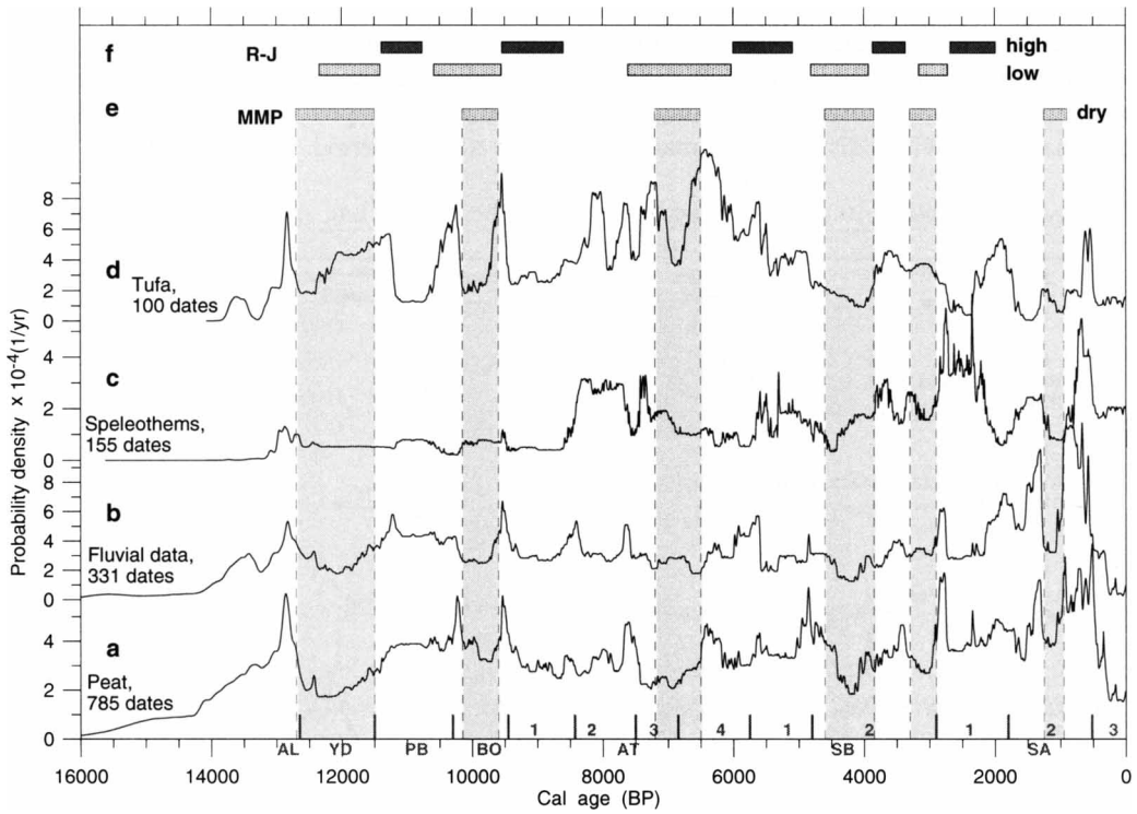
Figure 2 PDFs constructed for sets of 14 C dates: (a) 785 dates of peat samples; (b) 331 dates of samples connected with fluvial events; (c) 155 dates of speleotheims; (d) 100 dates of tufa samples. Periods with environmental conditions unfavorable for sedimentation (MMP) of all types of analyzed materials; dry periods (e) were established on the basis of coincidence of lowering of PDFs. For comparison, the reconstruction of lakes and mire levels for northern Poland R-J (Ralska-Jasiewiczowa 1989, after calibration) is presented in (f). A good agreement of establishing dry periods is seen. Small vertical lines at the bottom of the figure indicate borders of the Late Glacial and Holocene subdivisions (Pazdur 2004; Starkel et al. 2006).
