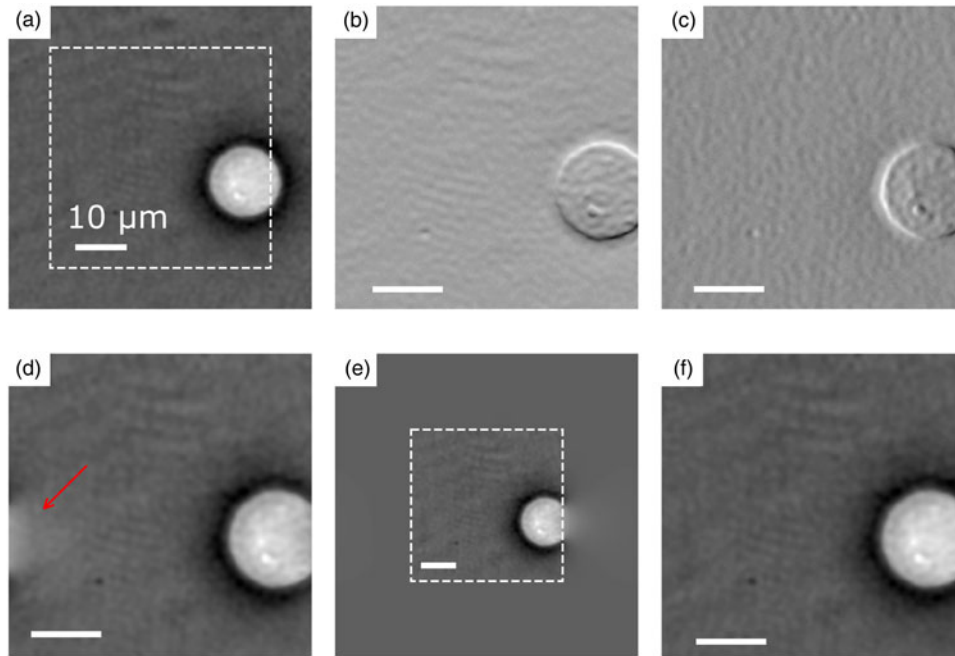
Fig. J.1. Boundary condition handling for DPC. (a) A test image, an optical holographic reconstruction of a biological cell in saline from Müller et al. (2018) along with the numerical derivatives of a cropped region (white dashed line) of the image in (b) and (c). (b,c) The DPC images. A DPC reconstruction from these produces (d), which has artifacts, most noticeably where indicated with a red arrow. The artifacts result from the boundary conditions implicitly assumed by the use of fast Fourier transforms. (e) The approach implemented in py4DSTEM, discussed in the body text, is to reconstruct on a padded grid [the original grid of (b) and (c) is indicated by the dashed outline]. The result of 10 iterations is shown in (f) which does not exhibit the same artifacts as (d).
