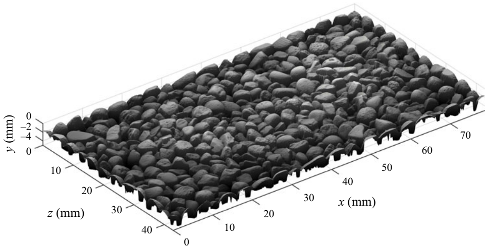
Figure 3. Illustration of periodic gravel roughness element; x , y and z are streamwise, wall-normal and spanwise coordinates, respectively.
