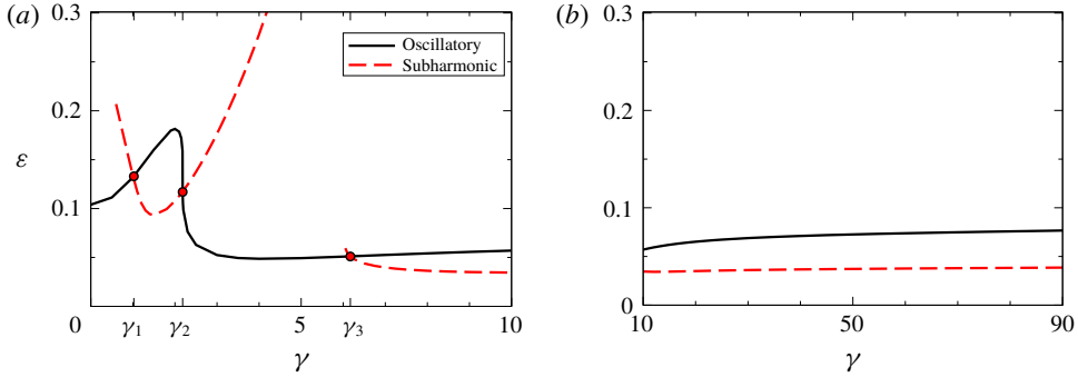
FIGURE 3. (Colour online) Stability diagram of transverse rolls for Pr = 0.025 with 0^\circ \leq \gamma \leq 10^\circ (a) and 10^\circ \leq \gamma \leq 90^\circ (b). The basic state in (2.2), stable for \epsilon < 0 (2.12), becomes unstable against the transverse rolls for \epsilon > 0 . These are stable below the lowest of the two lines, which determine either the OS instability at \epsilon = \epsilon_{OS} (solid line) or the SH instability at \epsilon = \epsilon_{SH} (dashed). The three crossing points of the two curves define the codimension-2 points \gamma_{1,2,3} .
