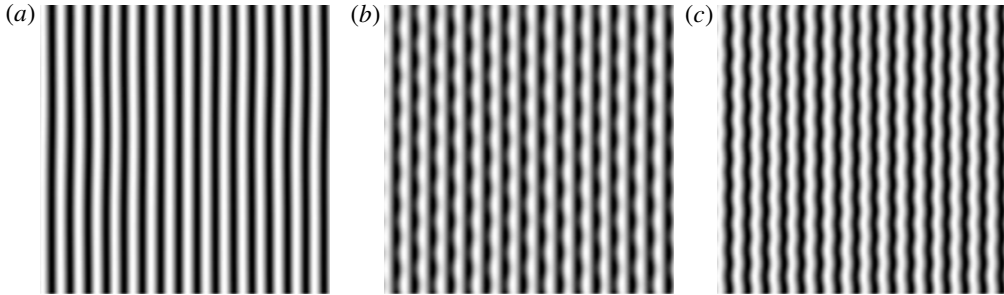
FIGURE 5. Basic patterns as in figure 4 for larger L_x = L_y = 16\lambda_c(\gamma) : (a) transverse rolls for \gamma = 50^\circ , \epsilon = 0.03 , \epsilon_0 = -0.8576 with \lambda_c = 2.293 . (b) SH pattern for \gamma = 50^\circ , \epsilon = 0.045 > 0.037 = \epsilon_{SH} , \epsilon_0 = -0.8556 . (c) Snapshot of an OS pattern for \gamma = 5^\circ , \epsilon = 0.055 > 0.049 = \epsilon_{OS} , \epsilon_0 = -0.2859 with \lambda_c = 2.104 (for details, see text).
