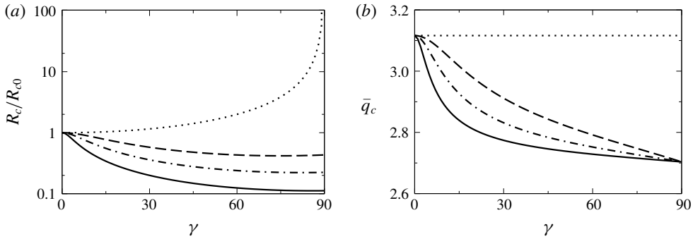
FIGURE 2. Linear instability of the ILC basic state for Pr = 0.025 (see (2.2)) as a function of the inclination angle \gamma with respect to rolls of wave vector \mathbf{q} = (q_x, q_y) = \bar{q}_c(\gamma, \psi)(\cos \psi, \sin \psi) at R = \bar{R}_c(\gamma, \psi) . (a) Reduced critical Rayleigh number \bar{R}_c(\gamma, \psi)/R_{c0} (logarithmic scale) with R_{c0} = 1707.8 . (b) Critical wavenumber \bar{q}_c(\gamma, \psi) . The solid lines correspond to the transverse rolls, where \bar{R}_c(\gamma, \psi = 0^\circ) is minimal. For the other \psi the following line styles are used: dotted for longitudinal rolls ( \psi = 90^\circ ), dashed for \psi = 75^\circ and dash-dotted for \psi = 60^\circ .
