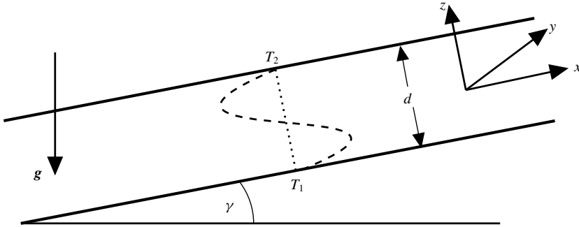
FIGURE 1. Fluid layer of thickness d inclined with an angle \gamma , heated from below and cooled from above with temperature difference \Delta T \equiv T_1 - T_2 > 0 . Driven by gravity g the cold fluid flows downwards near the top plate and the hot one flows upwards near the bottom plate leading to a cubic velocity profile across the fluid layer (see (2.2)).
