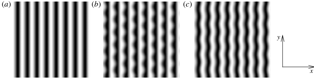
FIGURE 4. Midplane temperature plots in ILC for L_x = L_y = 8\lambda_c(\gamma) : (a) transverse rolls for \gamma = 3^\circ . (b) Stationary SH pattern for \gamma = 1.5^\circ . (c) Snapshot of an OS pattern for \gamma = 6^\circ (for details see text).
