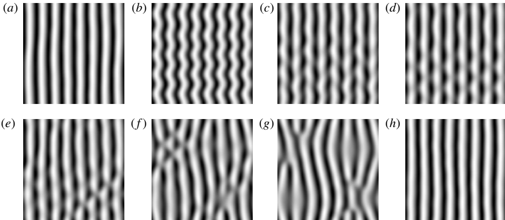
FIGURE 16. Heteroclinic orbit between OS, SH and transverse roll patterns for \gamma = 6.169^\circ , \epsilon = 0.08 and \epsilon_0 = -0.3419 with L_x = L_y = 8\lambda_c(\gamma) . The snapshots of h(x, y, t) are shown at times t = 0 (a), 140 (b), 690 (c), 890 (d), 1130 (e), 1300 (f), 1360 (g), 1490 (h) in units of t_v , increasing from left to right and from top to bottom.
