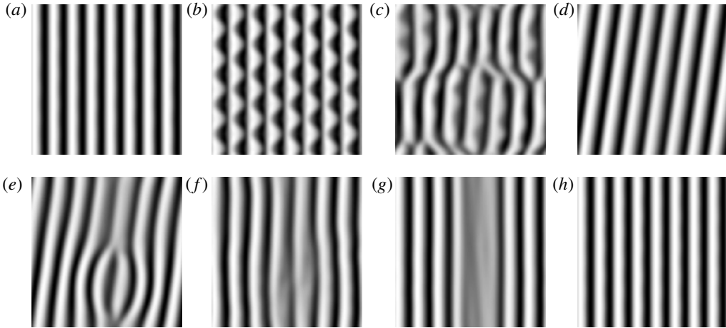
FIGURE 14. Heteroclinic cycle with subharmonic, transverse and oblique patterns from a DNS at \gamma = 1.5^\circ with L_x = L_y = 8\lambda_c(\gamma) at \epsilon = 0.165 ( \epsilon_0 = 0.0945 ). The pictures are sorted with increasing time t from left to right and top to bottom and correspond to t = 0 (a), 68 (b), 195 (c), 278 (d), 702 (e), 755 (f), 788 (g), 873 (h) in units of t_v .
