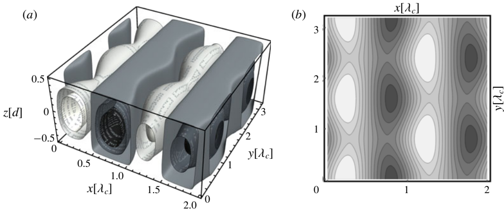
FIGURE 7. DNS for \gamma = 10^\circ , \epsilon = 0.05 , \epsilon_0 = -0.522145 , \lambda_x = \lambda_c(\gamma) = 2.175d with the periodicity lengths L_x = L_y = 8\lambda_x : (a) 3-D contour plot of \theta(x, y, z) for 0 \leq x \leq 2\lambda_x , 0 \leq y \leq 2\lambda_y = 2(8/5)\lambda_x ; (b) 2-D contour plot of the midplane temperature \theta(x, y, z=0) from panel (a).
