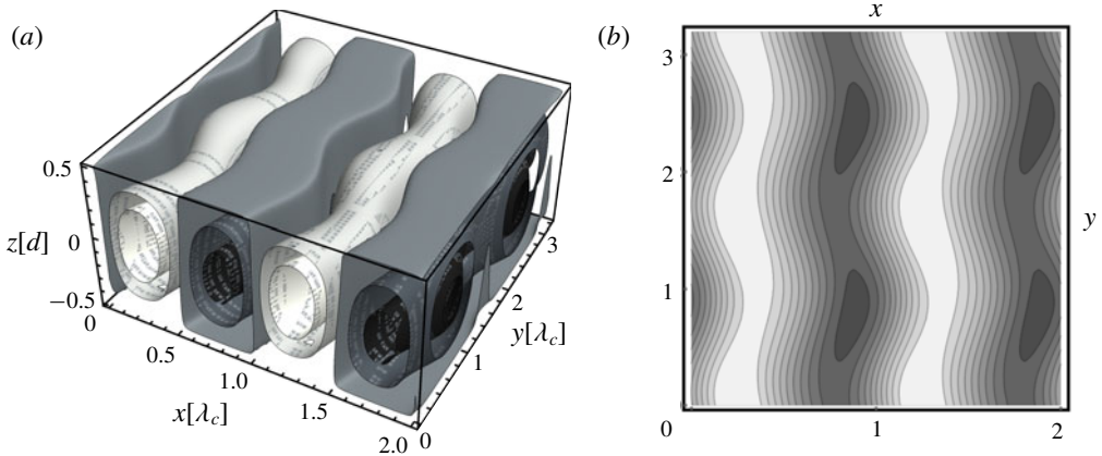
FIGURE 10. DNS for \gamma = 6^\circ , \epsilon = 0.07 , \epsilon_0 = -0.33836 , \lambda_x = \lambda_c(\gamma) = 2.175d with the periodicity lengths L_x = L_y = 8\lambda_x : (a) snapshot of a 3-D contour plot of the temperature \theta(x, y, z) for 0 \leq x \leq 2\lambda_x , 0 \leq y \leq 2\lambda_y = 2(8/5)\lambda_c and -d/2 < z < d/2 ; (b) 2-D contour plot of \theta(x, y, z) obtained from panel (a) for y=0 .
