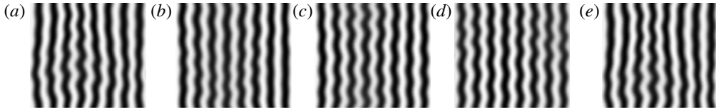
FIGURE 18. Complex travelling-wave pattern for \gamma = 0.5^\circ , \epsilon = 0.172 , \epsilon_0 = 0.163 , L_x = 8\lambda_c(\gamma) , L_y = 0.906L_x . The pictures are sorted increasing in time from left to right at t = 3728 (a), 3741 (b), 3779 (c), 3804 (d), 3851 (e) in units of t_v . For the travelling waves we find \omega = 1.62 .
