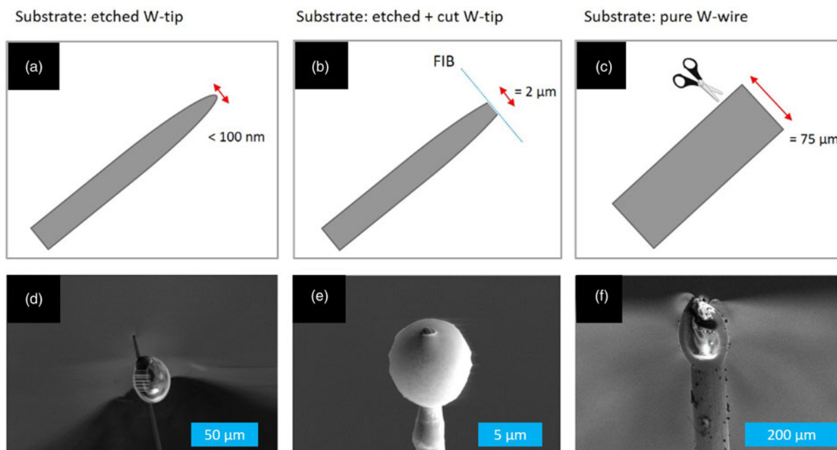
Fig. 6. Representative dipping results for W wires with different sample geometries in honey. (a) Etched W-tip, (b) W-tip that is etched and cut, and (c) a pristine W-wire.
