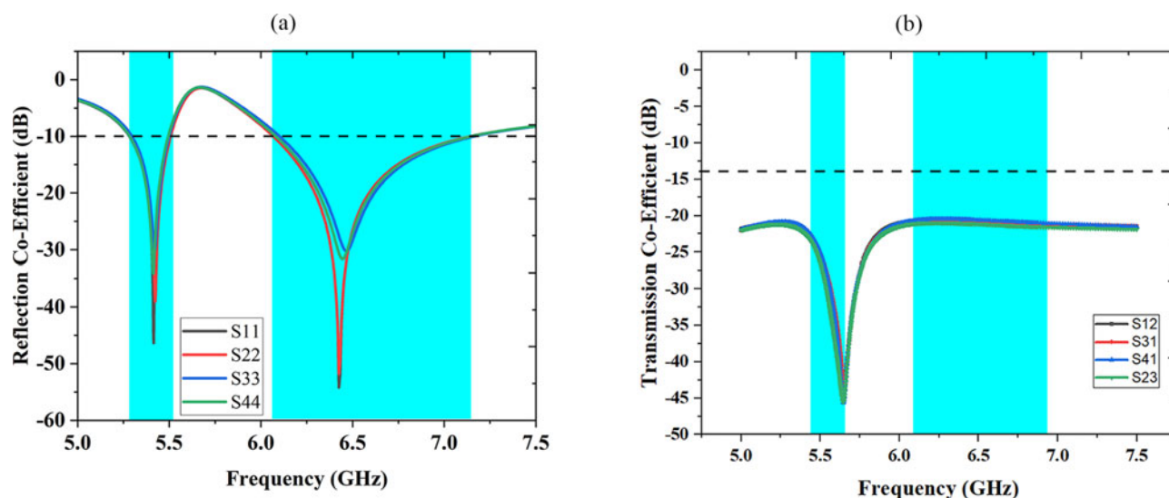
Figure 2. (a) S_{11} of Antenna 1-4, (b) S_{ij} of 4-port CSRR loaded antenna.
