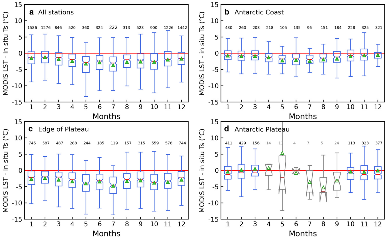
Figure 6. Temperature difference between cloud-screened MODIS LST and in situ T_s in each month at all stations (a), the stations on the Antarctic coast (b), the edge of the plateau (c) and the East Antarctic Plateau (d). Boxplots showed the 25th and 75th percentiles (boxes), the averages (green triangles) and the medians (orange short horizontal lines). The numbers at the top of the boxes were the paired amount of two types of LST observations in each month, and gray boxes in subplot (d) represented the months with fewer than 25 paired amounts. The red horizontal line represented the bias value equal to 0°C. The results cannot be extrapolated to other places without an AWS (equipped with cloud fraction).
