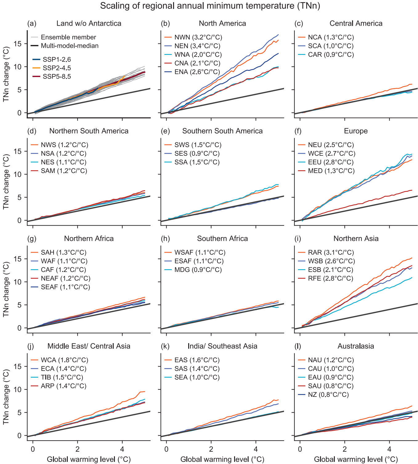
Figure 11.A.1 | As Figure 11.3 but for the annual minimum temperature (TNn).
