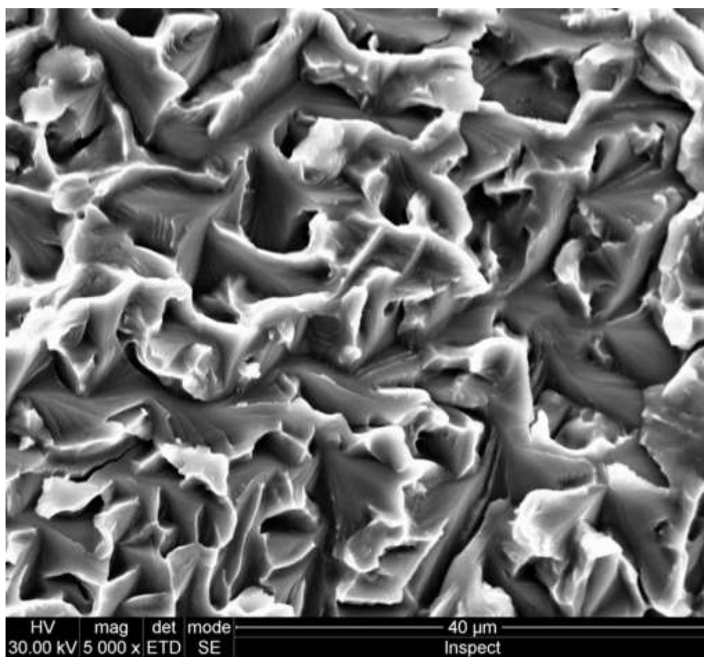
Figure 1. Fig.1 Fractograph of the core area of a tensile sample for the fiber with 0.4 mm diameter.
