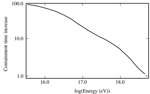
Figure 1 The result of a simulation of cosmic ray proton propagation from a hypothetical source close to the Galactic centre. The Galactic magnetic field is as described in Clay (2000) except that the random component has a rather constant mean strength and extends to 1 kpc above and below the Galactic plane. The random and regular fields have similar characteristic strengths of about 2 \mu\text{G} . The containment time is the extra factor of time required for the particles to leave the Galactic field, over that which results purely from their source directional distribution without any magnetic effects.
