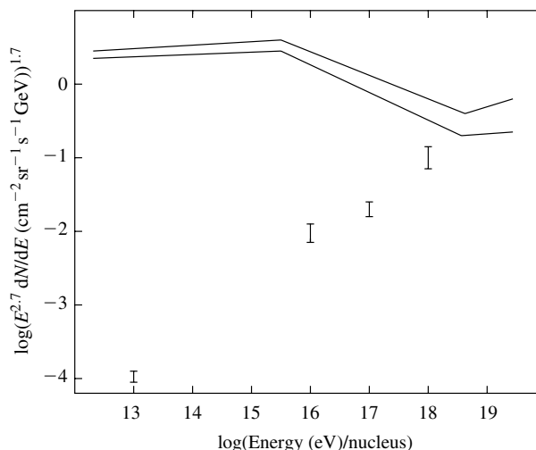
Figure 2 The cosmic ray energy spectrum (band of data — from Particle Data Group 1996) together with an unnormalised source spectrum (data with error bars) derived from the above spectrum using estimates of the Galactic containment time as a function of energy. The error bars are based on the spread in the energy spectrum alone, not including uncertainties in the containment time estimates. Shibata (1995) indicates that a power law with a differential index of approximately -2.3 applies to the source spectrum below 10^{15} eV.
