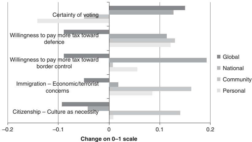
Fig. 4. Maximum effects of breadth of threats
