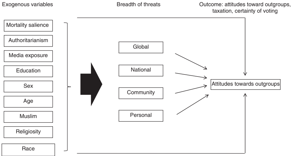
Fig. 1. The structural equation models
