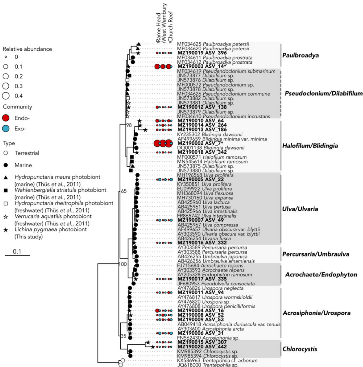
Fig. 5. 18S rDNA gene maximum likelihood phylogeny of Ulvophyceae associated with Lichina pygmaea ASVs significantly enriched in the intrathalline samples are indicated with *. Prefix ‘endo-’ refers to intrathalline (red circles) and ‘exo-’ refers to extrathalline (blue circles). Circle size is relative abundance. Node labels indicate bootstrap support values for main clades. Dashed lines next to clade names indicate paraphyletic clades.
