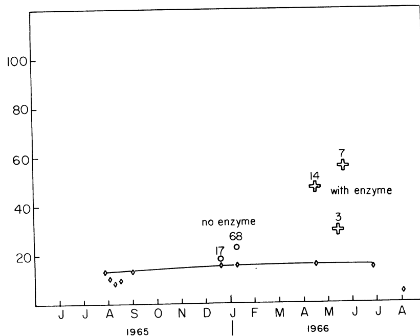
Fig. 2. C^{14} enrichment, in percent, of ocean water during 1965-66 at Los Angeles area beaches. Diamonds are direct measurements; their scatter is due to changing upwelling along the coast. However, it appears that C^{14} activity in surface ocean water is leveling off. Circles denote samples through which air has been bubbled for number of days stated. Crosses are samples containing carbonic anhydrase in the sea water and exposed to air for period marked.
