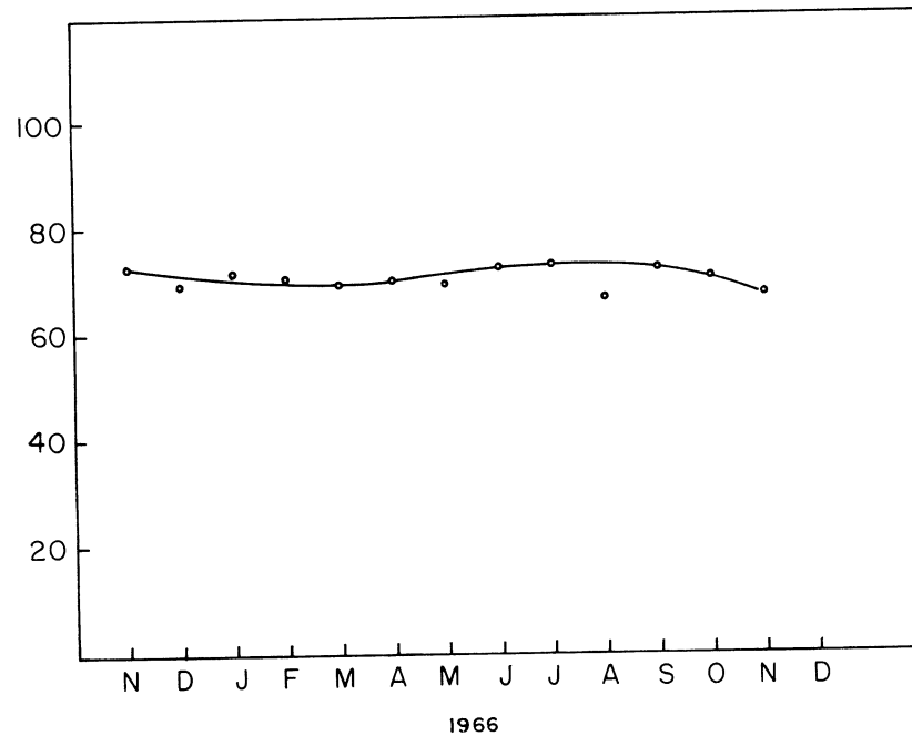
Fig. 1. C 14 enrichment in percent over NBS standard of atmospheric CO 2 during 1966 at China Lake, California (35° 37' N Lat, 117° 41' W Long).
