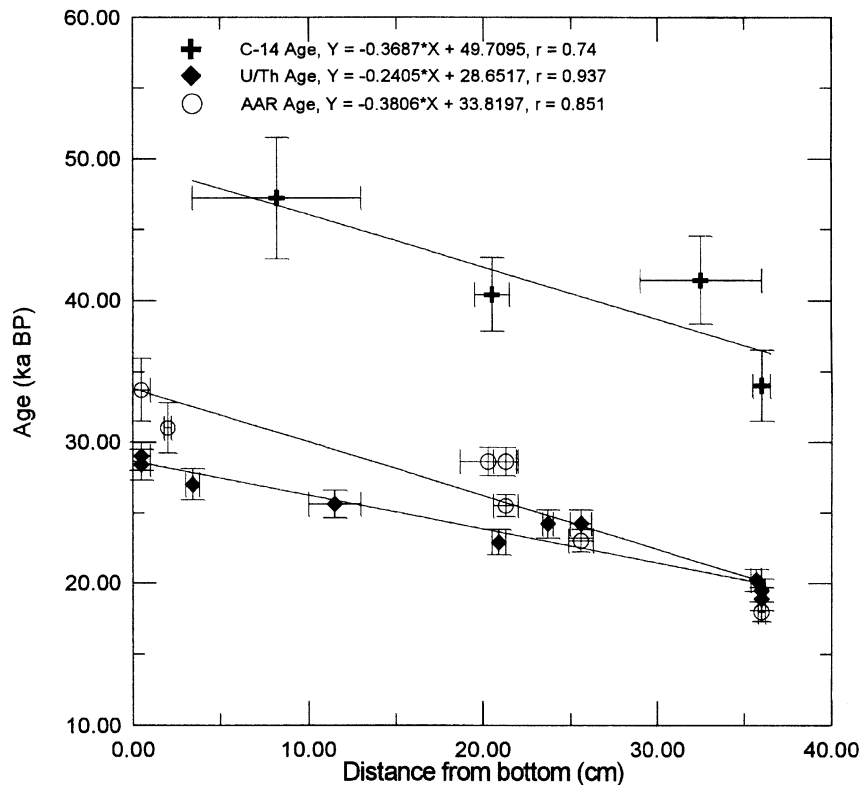
Figure 8 Results of ^{14}\text{C} , U/Th, and AAR dating of speleothem JW12. Samples were taken from different distances from the bottom. Straight lines are linear approximations of results by the least squares method (note the equation lines).
