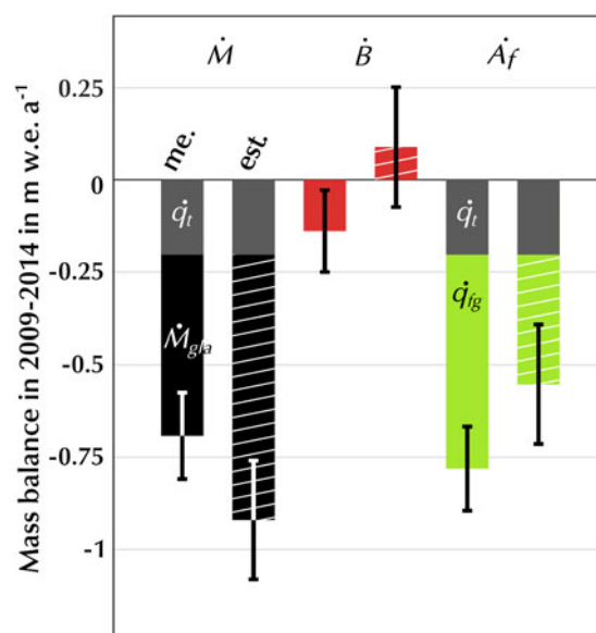
Fig. 4. Total mass balance from the geodetic method, \dot{M}_{me.} , from the mass budget method \dot{M}_{est.} , and its component the climatic mass balance, \dot{B} , and the frontal ablation, \dot{A}_f , for the validation period of 2009–2014 measured (flat bar) and estimated (hatched bar). The geodetic mass balance over glacierized area is in black, the climatic mass balance in red, the discharge at the terminus in green and the terminus position change contribution in grey. The mass loss by retreat of the terminus, \dot{q}_t , is distinguished from the mass loss by discharge through the terminus, \dot{q}_{fg} . The sum of the grey and green bars is the frontal ablation.
