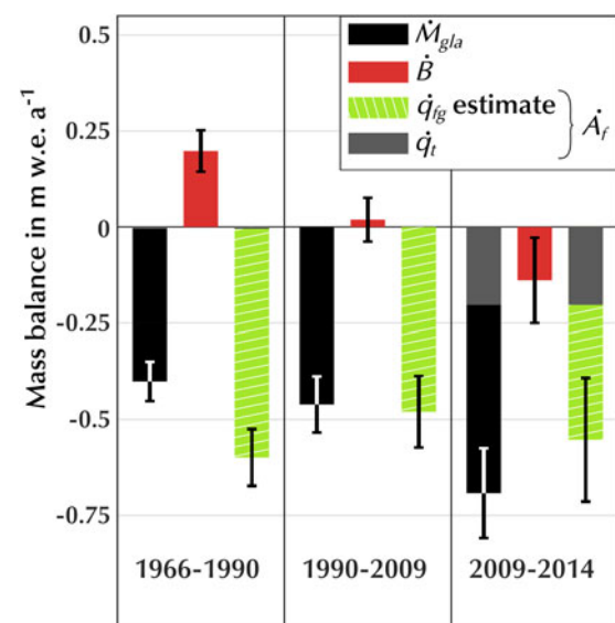
Fig. 6. Mass balance for three study periods measured with the geodetic method (black), separated between climatic mass balance (red), the estimated frontal ablation (green and grey). Grey shows the contribution of the terminus position retreat.
