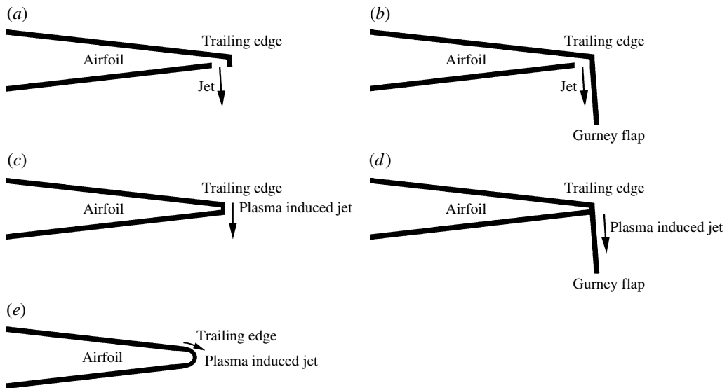
FIGURE 2. Sketch of the airfoil controlled by (a) jet (Traub et al. 2004), (b) Gurney flap with jet (Traub & Agarwal 2008), (c) plasma induced jet (Zhang et al. 2009), (d) Gurney flap with plasma induced jet (Feng et al. 2012) placed near the sharp trailing edge, and by (e) plasma induced jet (Zhang et al. 2010) near the round trailing edge.
