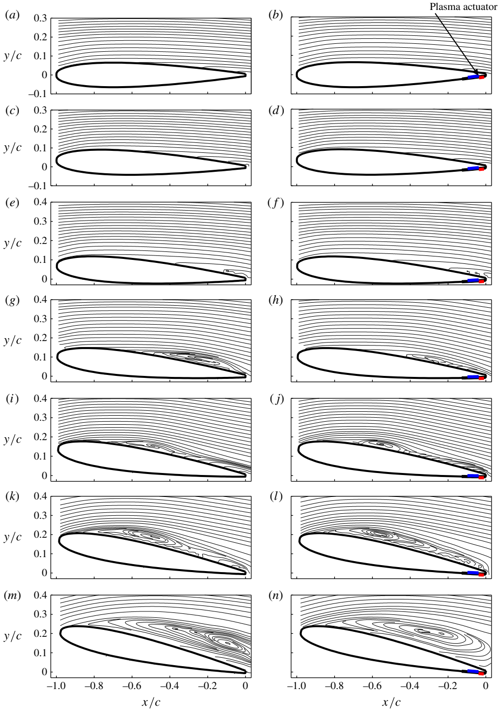
FIGURE 6. (Colour online) Time-averaged streamlines over an airfoil without ( a,c,e,g,i,k,m ) and with ( b,d,f,h,j,l,n ) plasma control at Re = 20\,000 , C_\mu = 1.9\% . ( a,b ) \alpha = 0^\circ ; ( c,d ) \alpha = 2^\circ ; ( e,f ) \alpha = 4^\circ ; ( g,h ) \alpha = 6^\circ ; ( i,j ) \alpha = 8^\circ ; ( k,l ) \alpha = 10^\circ ; ( m,n ) \alpha = 12^\circ .
