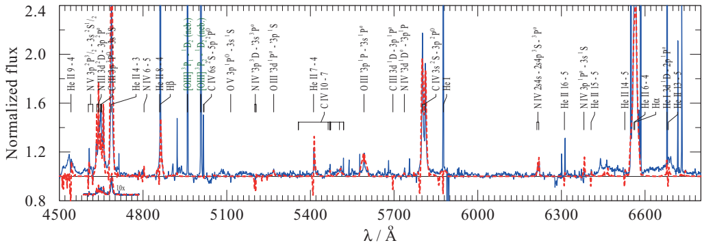
Figure 1. Optical spectrum of PB 8 - Observation (blue solid) vs. model (red dashed)
