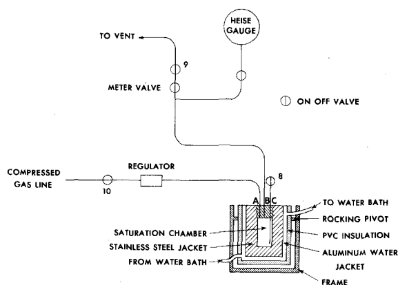
Figure 1. Equilibration system.
