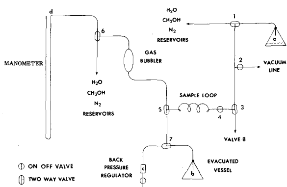
Figure 2. Sampling system.
