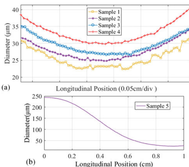
Figure 5. Diameter scanning of pump fiber tapers at different longitudinal positions for (a) Samples 1–4 (around the taper waist) and (b) Sample 5.
