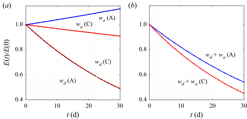
Figure 13. Temporal evolution of the vortex kinetic energy of cyclones (red) and anticyclones (blue) in experiments using the extended vorticity equation (3.7). Compare with the curves shown in figure 9: (a) A1, C1 (using w_d ) and A2, C2 (using w_a ). A1, C1 decay at the same rate (the curves are overlapped); (b) A3, C3 ( w_d + w_a ).
