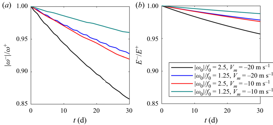
Figure 10. Temporal evolution of (a) the peak vorticity ratio |\omega^-|/\omega^+ between anticyclones and cyclones for different vortex amplitudes \omega_0 and wind speeds V_m , and (b) the corresponding kinetic energy ratio E^-/E^+ .
