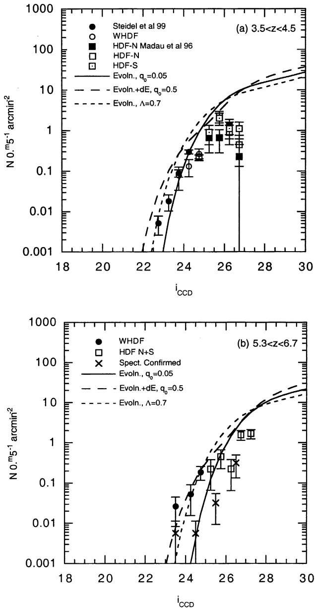
Figure 4. (a) The i_{\text{CCD}} number count of 3.5 \lesssim z \lesssim 4.5 B -dropout galaxies from the WHDF and HDF data, compared to our model predictions. The models fit well at bright magnitudes but are 5\times too high at faint magnitudes, indicating that luminous galaxies may form at z \gtrsim 4 while dwarfs form at z \lesssim 4 . (b) The i_{\text{CCD}} number count of 5.3 \lesssim z \lesssim 6.7 R -dropout galaxies from the WHDF and HDF data (Metcalf et al. 2000). The crosses are based on 6 spectroscopically confirmed z \approx 6 galaxies. The models show good agreement for the brighter galaxies, indicating that luminous galaxies form at z \gtrsim 6 .
