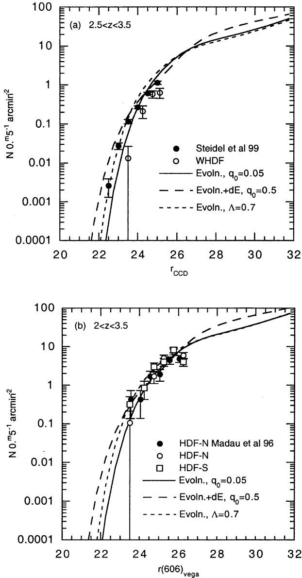
Figure 3. (a) The r_{CCD} number count of 2.5 \lesssim z \lesssim 3.5 ground-based UV dropout galaxies compared to our evolutionary model predictions. In the q_0 = 0.5 + dE case the contribution of the dE population can be seen at r > 25 . The WHDF data reasonably agrees with the data of Steidel et al. (1999) and overall we regard the agreement between the three evolutionary models and the data as excellent. (b) The r (F606W vega ) number count of 2 \lesssim z \lesssim 3.5 HDF UV-dropout galaxies compared to the same models as in (a). Again the agreement between these fainter data and the three evolutionary models is excellent.
