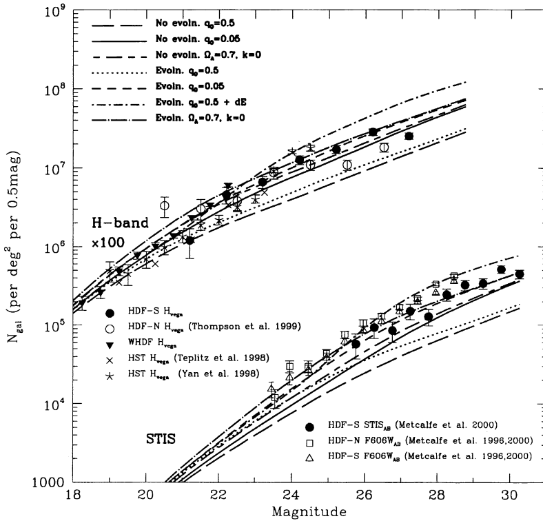
Figure 1. Lower points: HST STIS Hubble Deep Field South galaxy counts in the Clear passband from the data of Williams et al. (2000), analysed by techniques described elsewhere (Metcalf et al. 2000). Also shown are the HST WFPC-2 R (F606W) counts in the HDF-N,-S fields; the STIS counts are slightly lower than, but still statistically consistent with, these data in the range of overlap. Upper points: HST NICMOS HDF-N,-S galaxy count data in the infra-red H (F160W) passband from our analysis (Metcalf et al. 2000) of the data of Williams et al. (2000) in the case of HDF-S and directly from Thompson et al. (1999) in the case of HDF-N. The counts have been scaled upwards by a factor of 100 for clarity. HST NICMOS data from other authors are also shown (Teplitz et al. 1998; Yan et al. 1998). The WHDF data comes from a 20 hr exposure at the Calar Alto 3.5-m telescope using the \Omega' camera. The field-of-view is 7' \times 7' and the galaxy counts reach H = 22.5 . The models shown are those of Metcalfe et al. (1996) applied to both passbands (see text).
