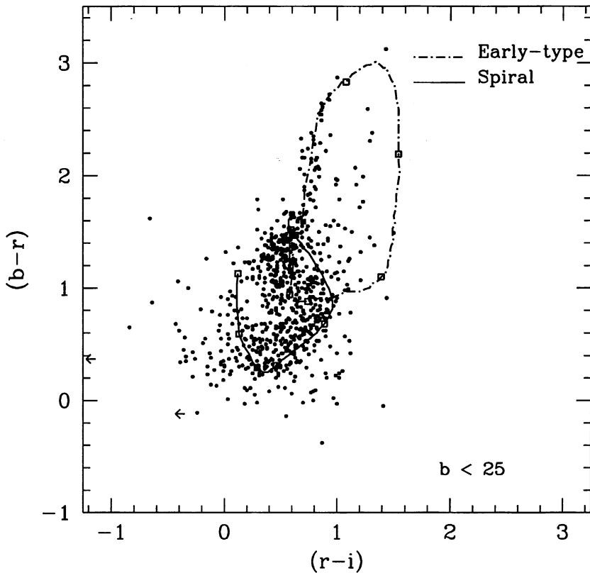
Figure 2. The B -limited r-i : b-r colour-colour diagram from the Herschel Deep Field data, showing the evolutionary tracks predicted from our Bruzual & Charlot models for essentially two galaxy types for 0 \lesssim z \lesssim 3 . Boxes indicate 0.5 z intervals. A plume of early-type galaxies can be seen which rise from b-r \approx 1.5 , r-i \approx 0.7 to redder b-r colours before turning bluewards again, as increasing star-formation at z \gtrsim 0.5 begins to affect the redshifted UV light. The spirals follow a horseshoe-shaped track below the early-types. This result clearly shows that there are just two main forms for the evolutionary behaviour of faint galaxies and the excellent fit of the Bruzual & Charlot models suggests that the main distinguishing feature is the star-formation rate, with \tau=2.5 Gyr assumed here for the early-types and \tau=9 Gyr for the spirals.
