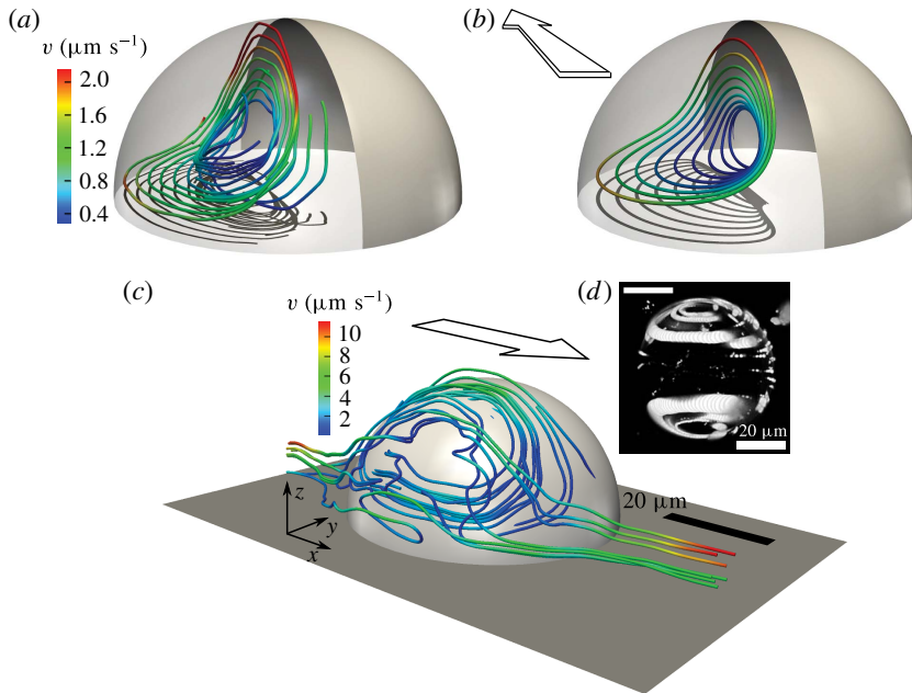
FIGURE 5. Velocity fields inside and outside a sheared vesicle. (a) Experimental and (b) theoretical interior flows are in excellent agreement. Exterior flows (c) exhibit closed streamlines, consistent with the circulation of phase-separated domains seen from confocal imaging (d). Arrows indicate flow directions. Reproduced from Honerkamp-Smith et al. (2013).
