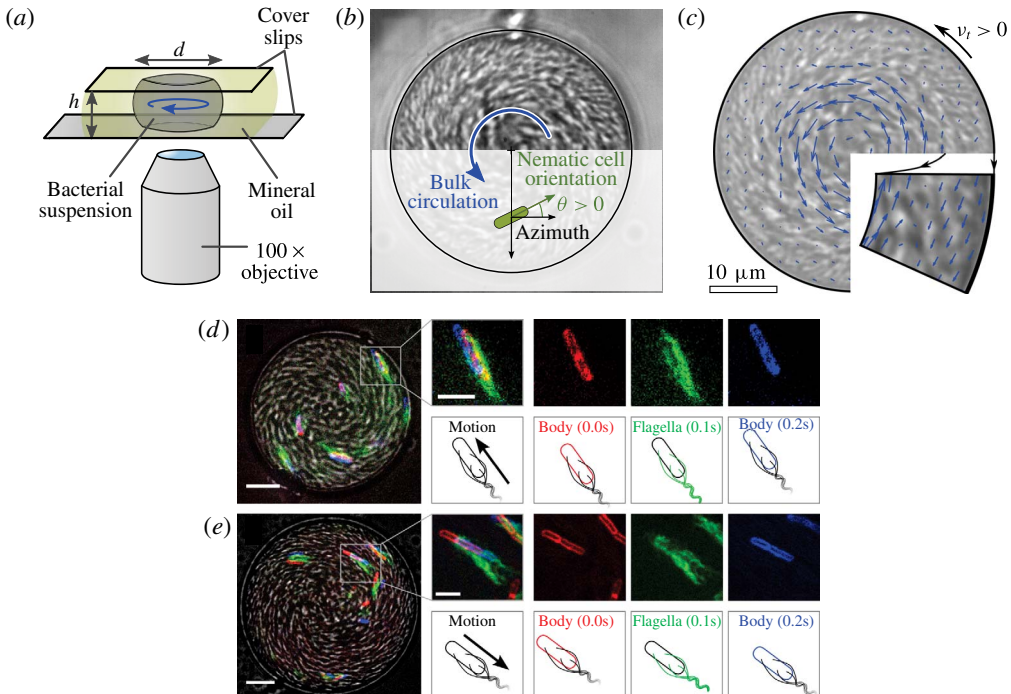
FIGURE 20. Confinement of a bacterial suspension. (a) A drop of bacterial suspension in a matrix of mineral oil. (b) Indication of bulk circulation in a drop, viewed from below. (c) PIV flow field in drop, with enlargement of boundary region showing edge current. Reproduced from Wioland et al. (2013). (d,e) Method for determining cellular orientation inside drop. Brightfield image with cell membrane (red at time t=0 and blue at t=0.2 s) and flagella (green at t=0.1 s) (d) Cell at the oil–water interface both points and moves to the top left corner. (e) Cell in bulk is pointing to the top left corner while moving overall in the opposite direction. (Scale bars: drop images, 10 \mu\text{m} ; individual bacteria, 5 \mu\text{m} .) Reproduced from Lushi et al. (2014).
