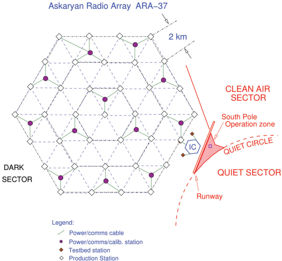
Figure 1. Planned layout of the 37 ARA stations with respect to the South Pole Station and associated sectors. The footprint of IceCube, which covers a square kilometer, is shown by the blue hexagon. The geographic South Pole is marked by the magenta square in the South Pole operation zone.
