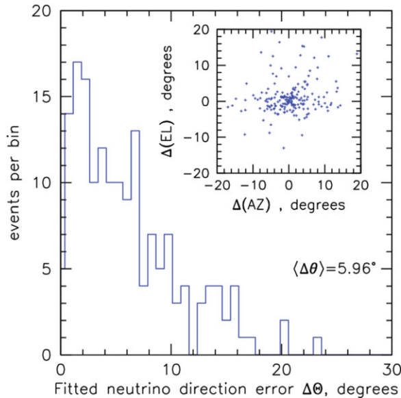
Figure 5. Distribution of fractional range errors in single-antenna-cluster reconstruction of neutrino interaction vertex. Distribution of polar angle errors for full reconstruction of the incoming neutrino direction, using vertex reconstruction, amplitude and polarization information. Inset: the 2-D distribution of reconstructed directions relative to true neutrino direction.
