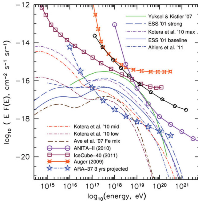
Figure 6. Compilation of sensitivity estimates from existing instruments, published limits, and a range of GZK neutrino models, along with the expected 3 year ARA sensitivity.
