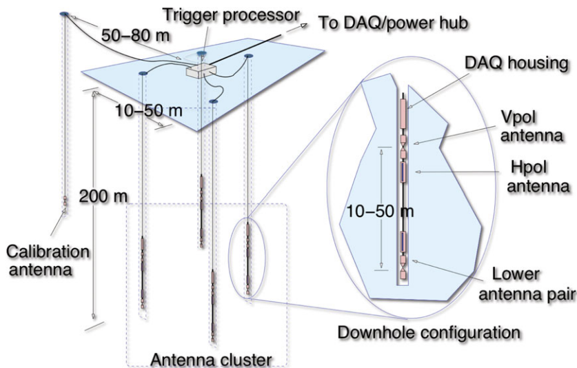
Figure 2. ARA Station layout and antenna cluster geometry.
