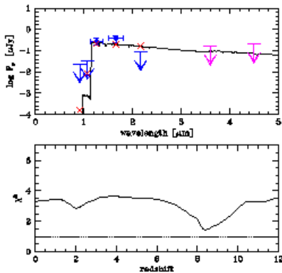
Figure 1. Best fit SED to the ACS, ISAAC and Spitzer observations (optical non-detections) of a high- z candidate from Richard et al. (2006) (top panel) and \chi^2 as a function of redshift, showing a redshift estimate of z \approx 8.4 .
