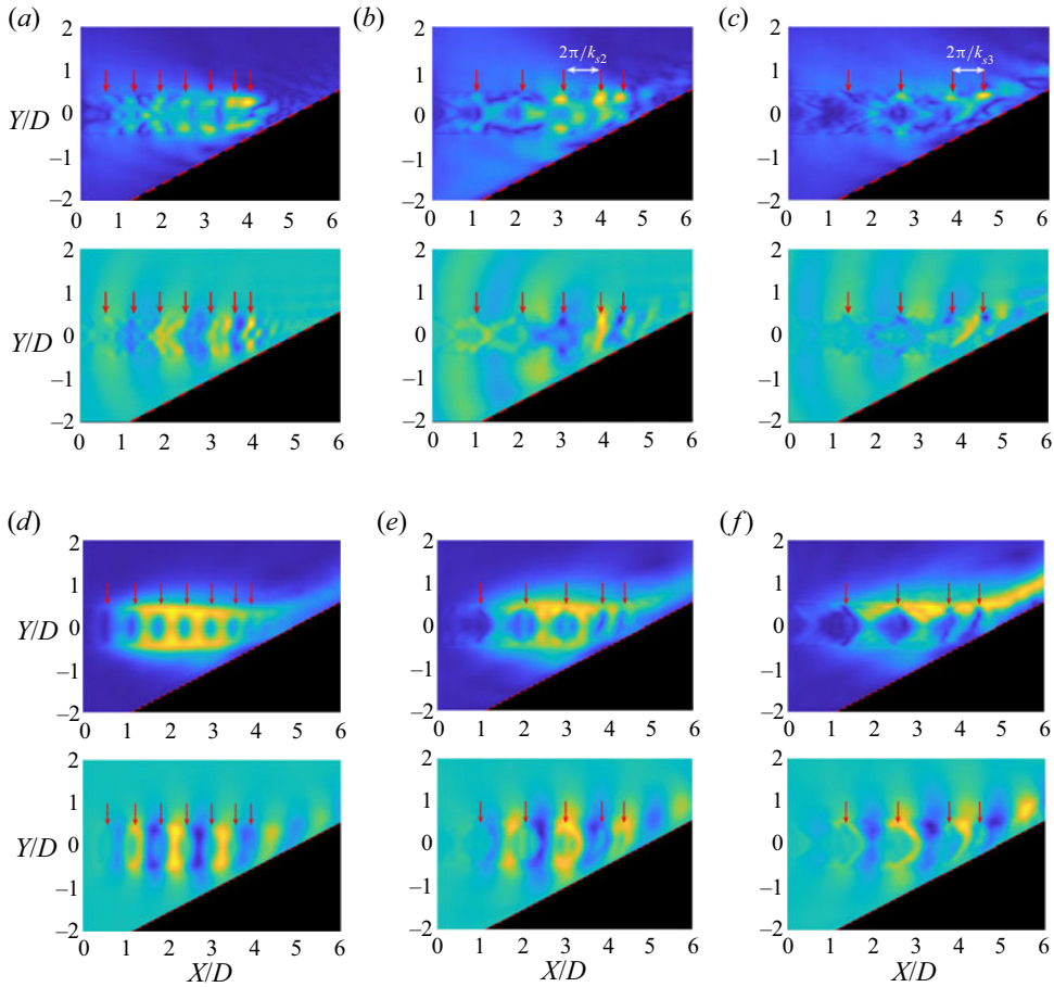
Figure 17. Approximately reconstructed upstream (a–c) and downstream (d–f) propagating waves at the screech frequencies for (a,d) the M_j = 1.12 jet (A1 mode), (b,e) the M_j = 1.28 jet (A2 mode), and (c,f) the M_j = 1.40 jet (A3 mode). The top image of each panel is the normalized amplitude field of waves. The colour scales range from 0 (blue) to 1 (yellow). The bottom image of each panel is the real part of the waves. Blue contours indicate negative values, and yellow contours indicate positive values. Red arrows indicate the axial positions of the shock reflection points at the jet shear layer.
