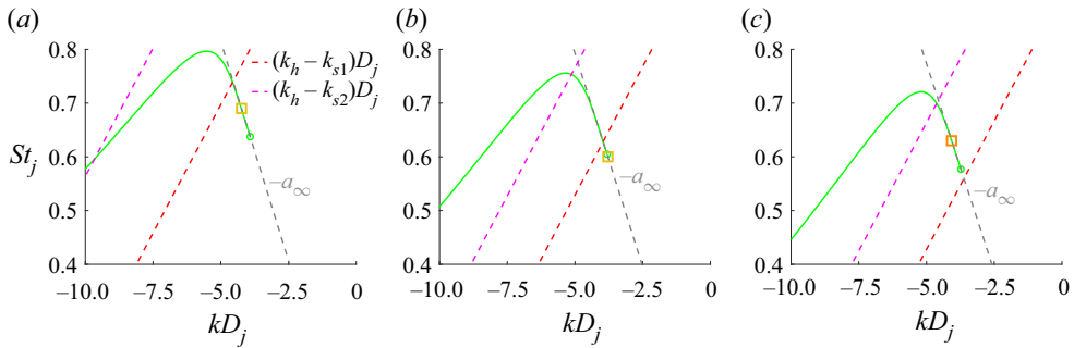
Figure 12. Dispersion relations of the upstream-propagating guided jet modes (0, 2) (green lines) for the jets at (a) M_j = 1.09 , (b) M_j = 1.12 , and (c) M_j = 1.16 . The red and magenta dashed lines respectively indicate the wavenumbers of k_h - k_{s1} and k_h - k_{s2} . The wavenumber of acoustic waves is represented by the grey dashed line. The yellow and orange squares respectively indicate the screech frequencies of the A1 and A2 modes.
