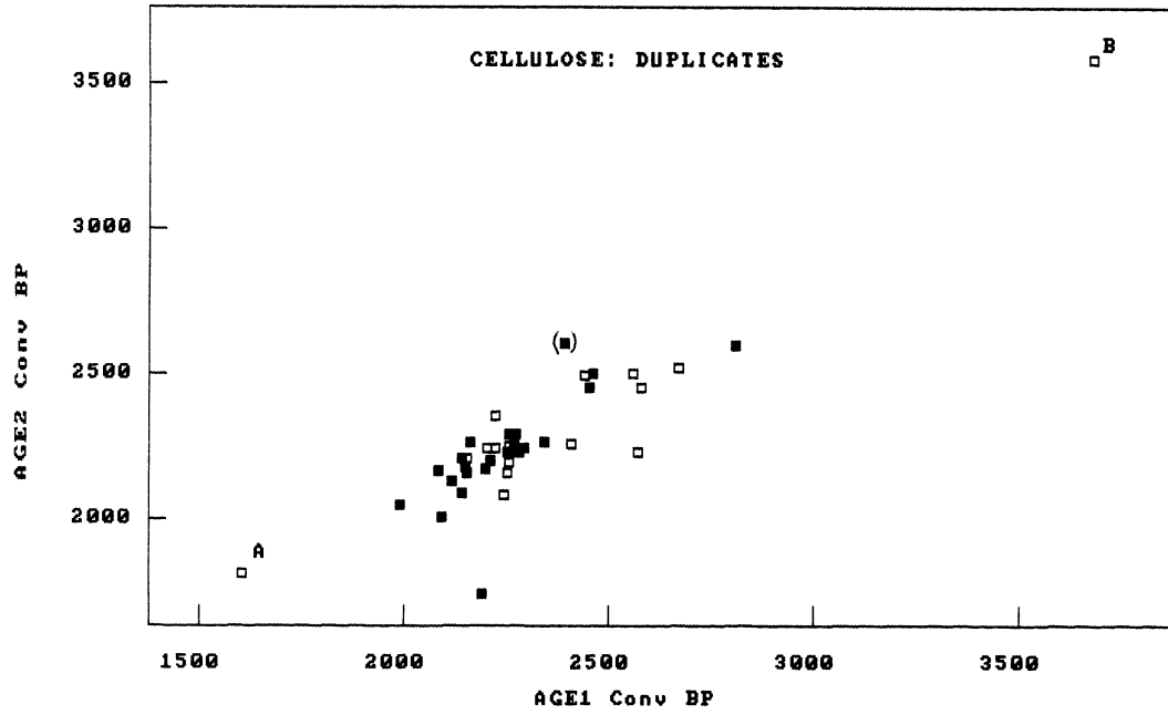
Fig 1. Results obtained on duplicate samples of cellulose, Stage 2. □ = LS labs, ■ = GC & AMS labs. Two distinctly outlying results are marked by A and B; the result of the Gliwice Lab is in parentheses.
