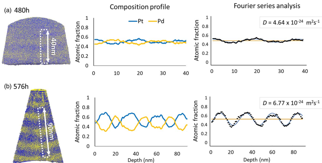
Fig. 11. The representative results of pre-alloyed multilayer samples annealed at 773 K for (a) 480 h and (b) 576 h.
