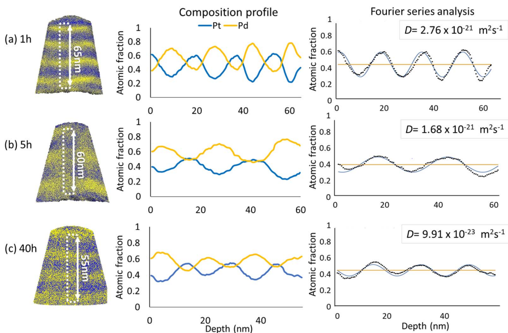
Fig. 6. The representative samples annealed at 873 K for (a) 1 h, (b) 5 h, and (c) 40 h.
