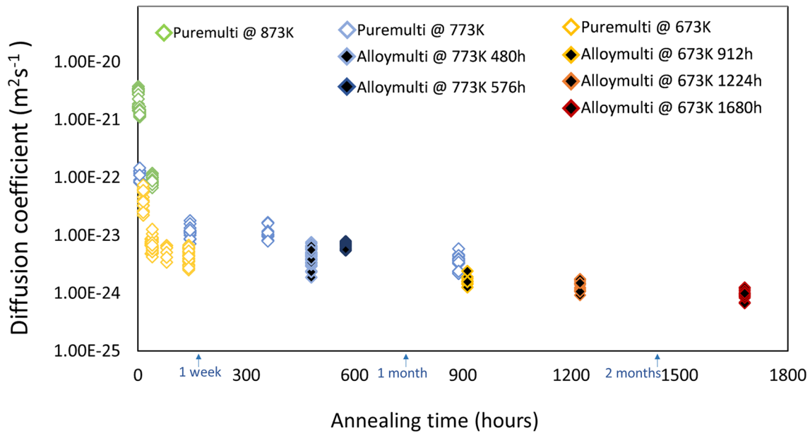
Fig. 13. Determined diffusion coefficients at corresponding annealing temperatures for pure multilayer samples (open diamond) and pre-alloyed multilayer samples (black color filled diamond).
