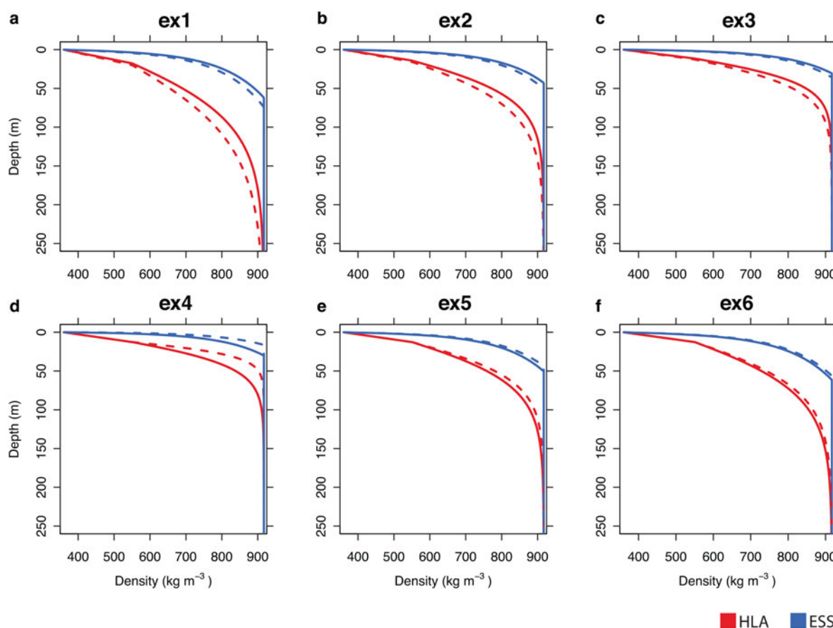
Fig. 11. Snow models and firm models both compute the densification of ice/air mixtures, but are calibrated under very different conditions in which different processes can be dominant. Here we compare depth-density profiles from the Essery and others (2013) snow model (ESS, blue) and from the Herron and Langway (1980) model (HLA, red) for the six firm experiments. Dashed curves are initial steady states, and solid curves are final states.
