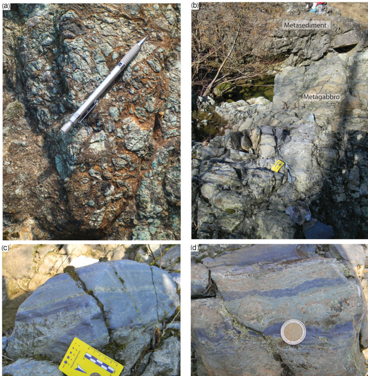
Figure 2. (Colour online) (a) Brecciated and carbonated serpentinites. (b) Overview of the metagabbro body and the glaucophanic metasediment lens. (c) Isoclinal fold ( D_2 ) inside the metagabbro body deforming a Na-amphibole-rich blue layer. (d) Detail of the layering in the metagabbro body and boudinage of the Ca–Na-pyroxene-rich green layer. Pen for scale is 15 cm long; coin is 2.5 cm diameter.
