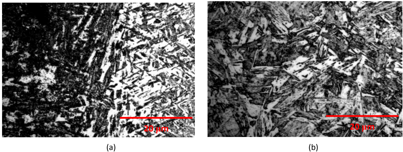
Figure 1. Micrographs of welded sample with no preheat, (a) near fusion (b) weld
