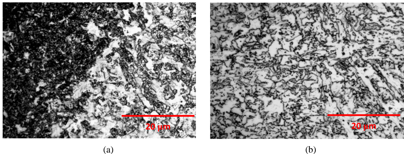
Figure 2. Micrographs of welded sample at 200°C preheat, (a) near fusion (b) weld
