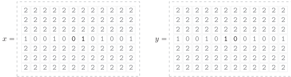
FIGURE 7. An indistinguishable, recurrent, but not uniformly recurrent asymptotic pair (x, y) given by the two characteristic Fibonacci words (\alpha = (\sqrt{5} - 1)/2) in the central row.
