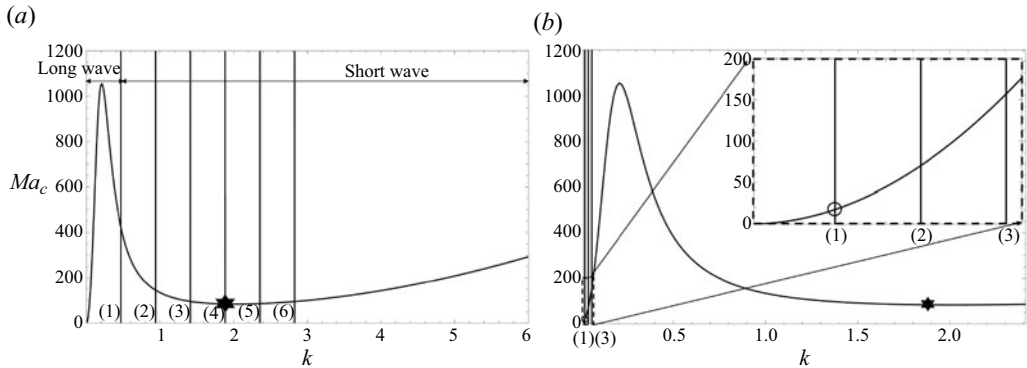
Figure 2. Critical Ma versus k curves, marking allowable wavenumbers k = 2m\pi/W with vertical lines. The numbers between parentheses correspond to m . Here (a) 1/W = 0.075 and (b) 1/W = 0.003 . The inset in (b) is a magnification of the low wavenumber range.
