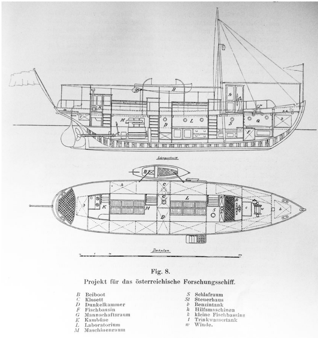
Figure 3. Draft for the construction of an “Austrian research vessel,” launched under the name Adria in 1908. It was the monarchy’s first ship designed explicitly for scientific purposes, and in addition to seawater aquariums and a laboratory with instruments and microscopy stations, it provided accommodation for six researchers and five crew members. Carl Cori, Ein österreichisches Forschungsschiff (Vienna, 1906), 19.
