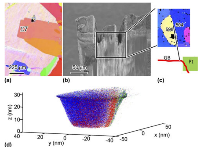
FIG. 29. (a) EBSD map showing partially recrystallized grain located away from the nucleation site. Larger, darker grains are of grain boundaries with \Sigma 7 tilt character at their mobile leading edge. (b) Secondary electron image of the specific area containing the \Sigma 7 grain boundary. (c) EBSD inverse pole figure map of the area designated in the box in the center image. (d) Schematic diagram showing the \Sigma 7 grain boundary (plan view) and the location of the Pt "cap" to be applied before milling. From Ref. 268. Copyright Elsevier, reproduced with permission.
