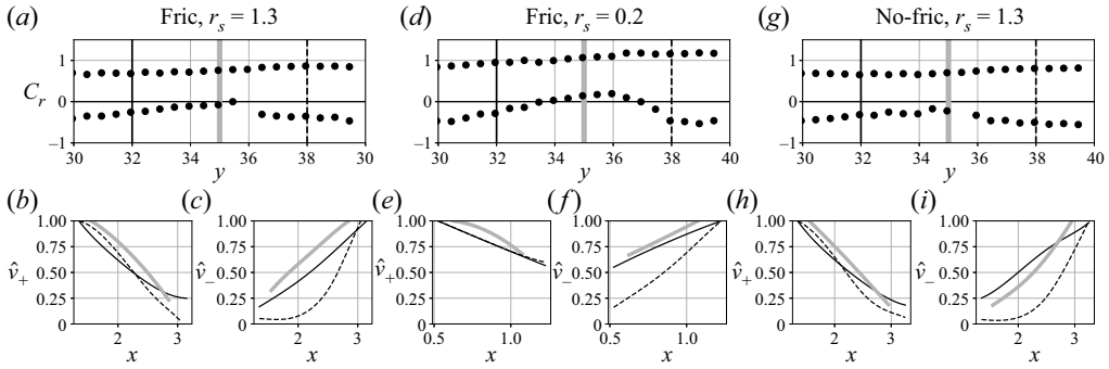
Figure 9. The left ( a–c ), middle ( d–f ) and right ( g–i ) panels show modal results calculated from time-mean model output from the friction experiment, friction experiment for a narrow-channel case and no-friction experiment, respectively. Here, h_s = 0.6 for all three experiments. The top panels show the phase speeds ( c_r , the subscript ( r ) denotes the real component) for the lowest modes along the channel. The bottom panels show the cross-sectional structure of the eigenfunction \hat{v} normalized by its maximum for the lowest mode. The solid black curves, thick grey curves and dashed black curves represent modes at an upstream section y = 32 , the sill y = 35 and a downstream section y = 38 , respectively (see a, d, g ). For a pair of frontal wave modes, \hat{v}_+ and \hat{v}_- correspond to waves that are downstream propagating and upstream propagating relative to the background flow, respectively.
