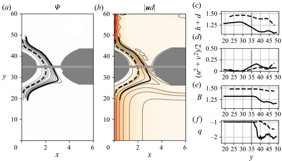
Figure 10. Time-averaged results from the friction experiment for the Samoan Passage topographic parameters ( r_s = 1.3 , h_s = 0.6 ). ( a ) Transport streamlines with \Psi ranging between -0.5 and -0.42 (dashed black contours) and between -0.38 and -0.28 (solid black contours). The contour interval is 0.02 . ( b ) The magnitude of transport |ud| (colours) and the interface height d + h (thin black contours). The thick dashed black curves and solid black curves in ( a ) and ( b ) represent streamlines \Psi = -0.46 and \Psi = -0.3 , respectively. Flow properties along the two streamlines are shown in ( c–f ). The grey horizontal lines in ( a, b ) and vertical lines in ( c–f ) mark the location of the sill.
