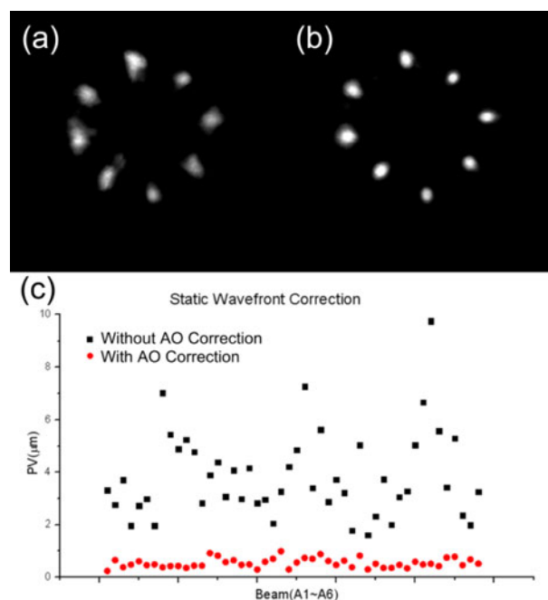
Figure 16. Correction effect of the AO system. (a) and (b) give the 3\omega focal spots on the target before and after AO correction, and (c) shows the wavefront distortion value of the whole 48 beamlines before and after AO correction.
