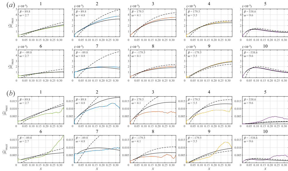
Figure 15. Growth of different modes ( \omega, \beta ) corresponding to L = 0.01 . Colour lines represent DNS data, dashed lines projection over the optimal and solid black lines LBLE results using DNS profile as initial condition. See figure 10 for modes numbering. Here (a) Tu = 0.5\% and (b) Tu = 3.0\% .
