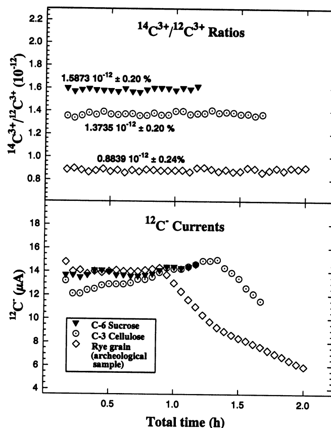
Fig. 3. Long-term measurements on single targets. The numbers shown in the top half of the figure indicate the 14 C 3+ / 12 C 3+ ratios (normalized to δ 13 C = -25‰) and the relative standard deviation of the mean. The corresponding relative statistical errors of the mean are 0.19%, 0.18%, and 0.22% for the C-6 Sucrose, the C-3 Cellulose, and the rye grain target, respectively.
