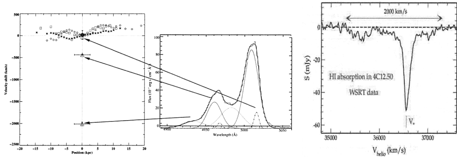
Figure 1. Left Radial velocity profile of the extended gaseous halo of 4C12.50. Key: *, \diamond and \square : highly extended [O II] emission (narrowest component); \bullet : H I 21-cm absorption; \triangle : 3 components of [O III] in the nucleus. The [OIII] profile with the components from the fit is also shown. Right The H I absorption profile detected in 4C 12.50 from the WSRT observations. The spectra are plotted in flux density (mJy) against optical heliocentric velocity in \text{km s}^{-1} .
