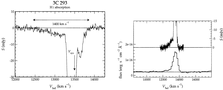
Figure 2. Left A zoom-in of the H I absorption spectrum of 3C 293 clearly showing the broad H I absorption. The spectrum is plotted as flux (mJy) against optical heliocentric velocity in \text{km s}^{-1} . Right Comparison between the H I absorption (top) and the [OII]3727Å (bottom, from Emonts et al. in prep.) profiles in the radio galaxy 3C 293. The similarity of the broad, blueshifted wing in the two profiles is evident.
