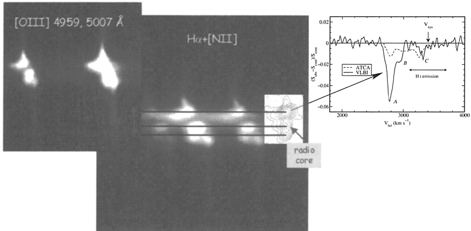
Figure 3. Left: a zoom-in of the [OIII] and H\alpha + [NII] lines in the Seyfert IC 5063. The radio image on a similar scale is also shown. The highly blueshifted component close to the bright radio lobe is clearly visible. Right: H I absorption profile profile detected against the NE radio lobe (from Oosterloo et al. 2000).
