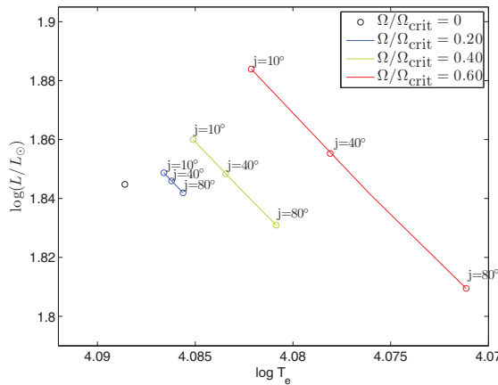
Figure 2. Luminosity and effective temperature of the 2.9 M_{\odot} model aged of \sim 20 Myr in the cases of no rotation and rotation at 0.20, 0.40 and 0.60 \Omega_{\text{crit}} , for inclinations j from 10^{\circ} to 80^{\circ} .
