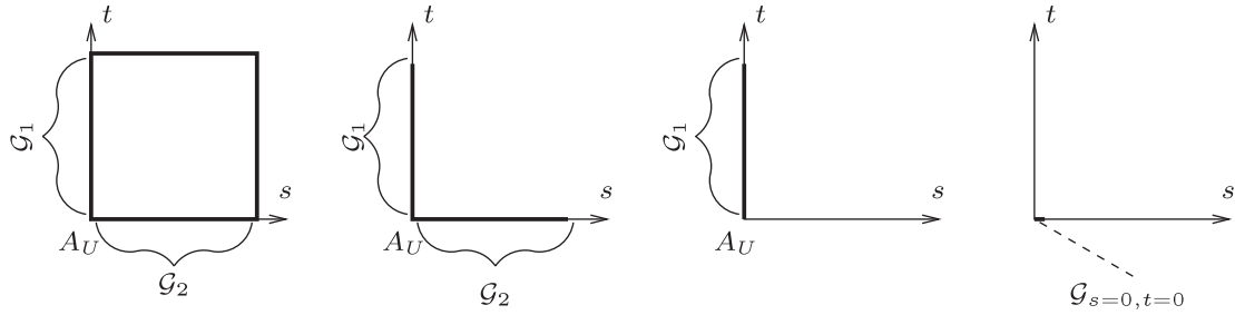
FIGURE 2. Successive restrictions of \mathcal{G} .
