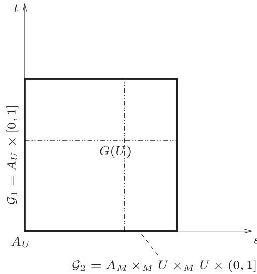
FIGURE 1. The groupoid \mathcal{G} .
