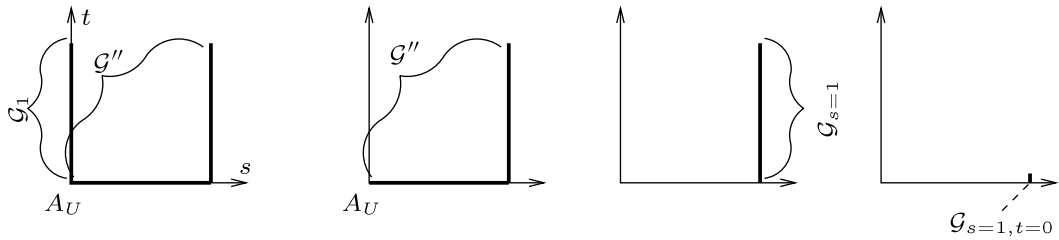
FIGURE 3. Other successive restrictions of \mathcal{G} .
