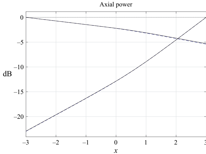
FIGURE 10. Axial acoustic power 10 \log_{10} |\mathcal{P}| in dB of right-running mode 2 and left-running mode -2 as a function of x .
