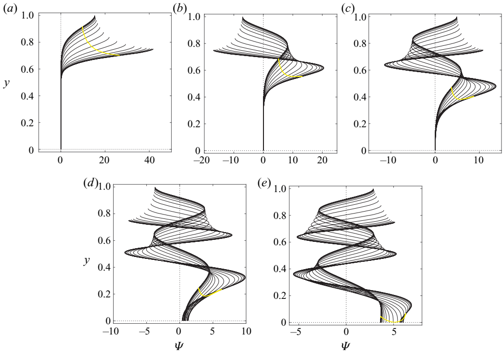
FIGURE 6. Left-running n th-order modal functions \Psi_n(X, y) for \omega = 15 , as a function of y - g for varying X . \Psi_{-6} becomes cut-off and is not included. (a) \Psi_{-1} . (b) \Psi_{-2} . (c) \Psi_{-3} . (d) \Psi_{-4} . (e) \Psi_{-5} .
