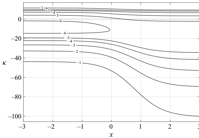
FIGURE 7. Axial wavenumbers \kappa_1, \dots, \kappa_{-1} (from top to bottom) as a function of x . \kappa_6 and \kappa_{-6} become cut-off and merge together at x = -0.055 .
