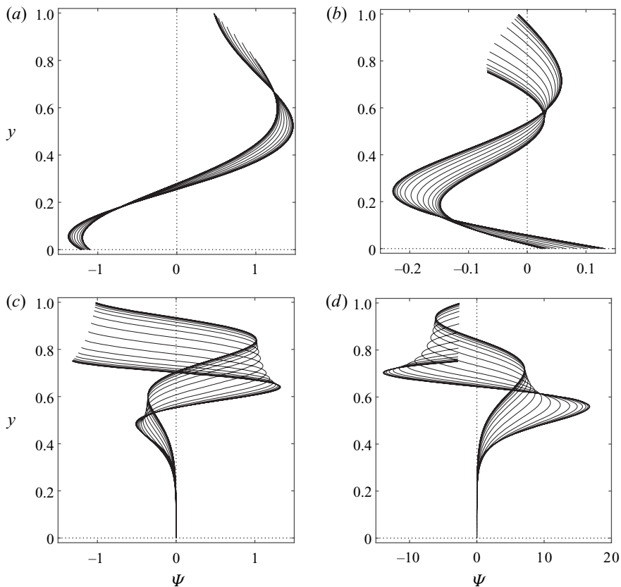
FIGURE 9. Real and imaginary parts of modal functions \Psi_{\pm 2}(X, y) for \omega = 15 , Z = 1 + 2i , as a function of y - g for varying X . (a) \text{Re}(\Psi_2) . (b) \text{Im}(\Psi_2) . (c) \text{Re}(\Psi_{-2}) . (d) \text{Im}(\Psi_{-2}) .
