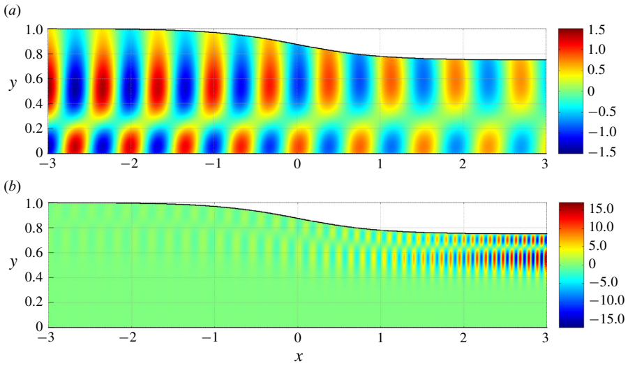
FIGURE 8. Pressure field snapshots (orders \pm 2 ) for \omega = 15 and Z = 1 + 2i . (a) \kappa_2 = 9.56 - 0.84i, \dots, 7.99 - 0.13i . (b) \kappa_{-2} = -30.25 + 0.38i, \dots, -61.22 + 0.53i .
