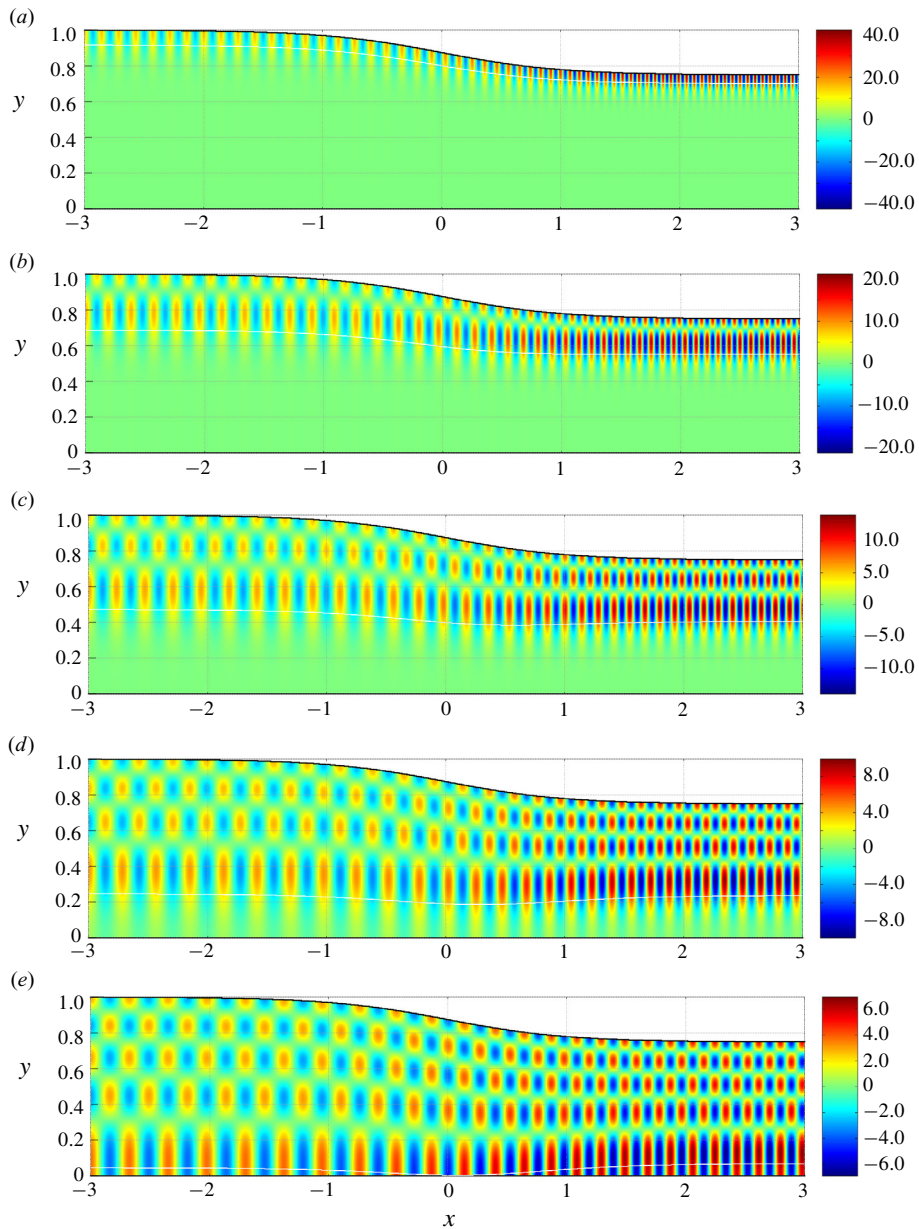
FIGURE 4. Pressure field snapshots (order -1, \dots, -5 ) for \omega = 15 and \mathcal{P} = -1 (left running). (a) \kappa_{-1} = -43.78, \dots, -100.04 . (b) \kappa_{-2} = -32.82, \dots, -69.40 . (c) \kappa_{-3} = -26.55, \dots, -52.84 . (d) \kappa_{-4} = -22.13, \dots, -41.69 . (e) \kappa_{-5} = -19.27, \dots, -34.44 .
