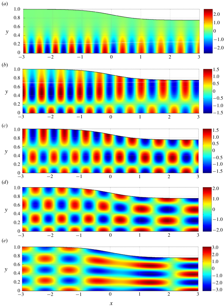
FIGURE 3. Pressure field snapshots (order 1, \dots , 5) for \omega = 15 and \mathcal{P} = 1 (right running). (a) \kappa_1 = 11.47, \dots, 9.33 . (b) \kappa_2 = 9.71, \dots, 8.27 . (c) \kappa_3 = 8.77, \dots, 6.63 . (d) \kappa_4 = 7.07, \dots, 3.34 . (e) \kappa_5 = 4.01, \dots, -2.26 .
