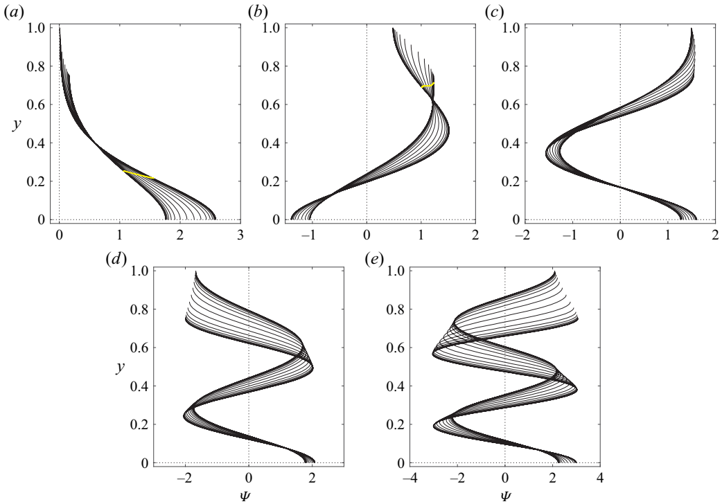
FIGURE 5. Right-running n th-order modal functions \Psi_n(X, y) for \omega = 15 , as a function of y - g for varying X . \Psi_6 becomes cut-off and is not included. (a) \Psi_1 . (b) \Psi_2 . (c) \Psi_3 . (d) \Psi_4 . (e) \Psi_5 .
