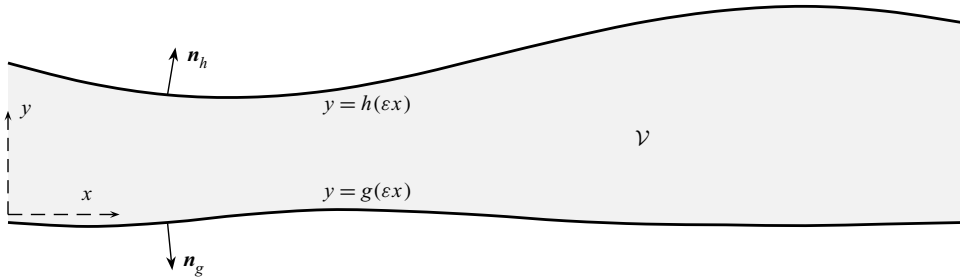
FIGURE 1. Sketch of geometry: two-dimensional slowly varying duct.
