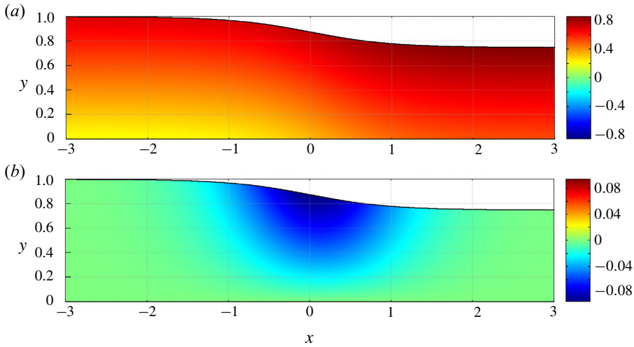
FIGURE 2. Mean flow in x, y -domain. (a) Mean flow U . (b) Mean flow V .
