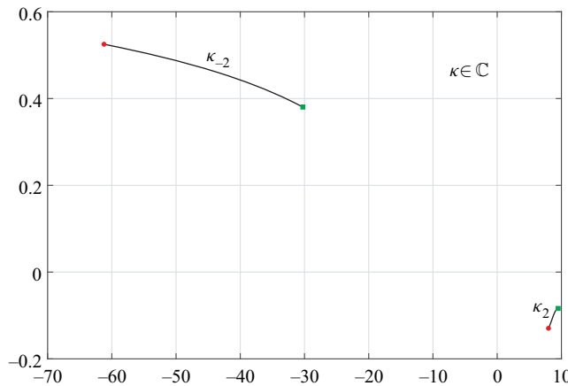
FIGURE 11. Complex axial wavenumbers \kappa_{\pm 2} varying from x = -3 (■, green) to x = 3 (●, red).
