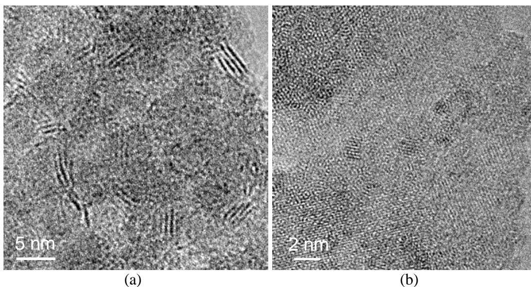
Figure 2. HR-TEM images showing a) edge-based MoS 2 structures on the Al 2 O 3 surface and b) some lattice lines in a thin region of the Al 2 O 3 sheet.
