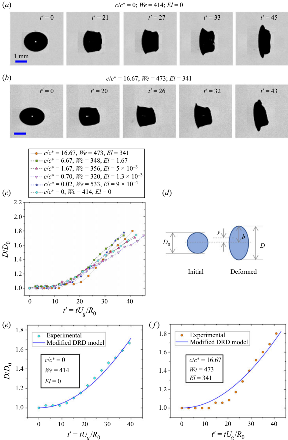
Figure 5. Effect of liquid elasticity on droplet deformation dynamics. (a,b) Experimental images showing aspect ratio evolution for water and polymeric droplet with c/c^* = 16.67 . (c) Temporal variation of droplet deformation for water and polymeric droplets with different c/c^* at comparable We . (d) Schematic of a spherical droplet deforming into the shape of an oblate spheroid. Comparison of experimental deformation with the modified DRD model for c/c^* values of (e) 0 and (f) 16.67.
