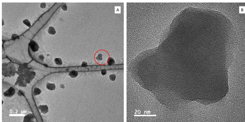
Figure 1. [A] Low magnification TEM image of C 60 particles on C film [B] HR image of the C 60 particle indicated in Fig 1[A]
