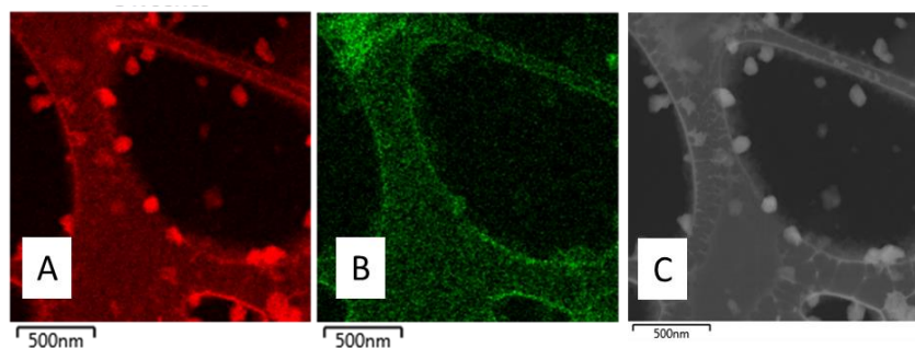
Figure 3. EDS Map [A] Carbon [B] Oxygen [C] Low magnification STEM Image.
