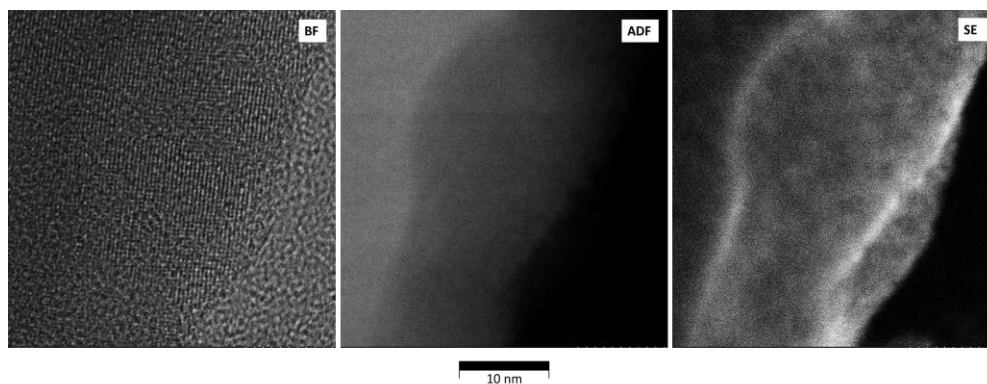
Figure 2. Simultaneous STEM BF/ADF/SE Imaging. The lattice fringes can be seen in the BF image.
