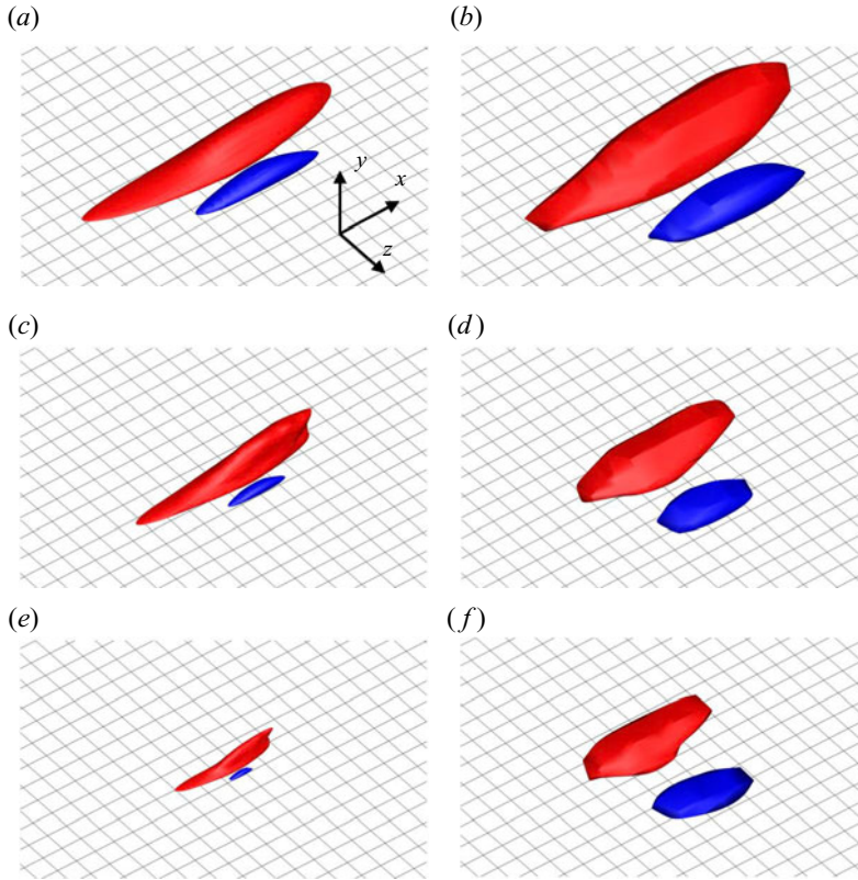
Figure 15. Conditionally averaged near-wall three-dimensional turbulence structures of the Q2–Q4 pair. Blue iso-surface, Q2 (low-speed streaks); red iso-surface, Q4 (high-speed streaks). The iso-surfaces are defined at \hat{u}''/\bar{u}_\tau = -1.5 for Q2, and \hat{u}''/\bar{u}_\tau = 1.5 for Q4. (a) DNS ( Re_\tau \approx 700 ), (b) WMLES ( Re_\tau \approx 700 ), (c) DNS ( Re_\tau \approx 1250 ), (d) WMLES ( Re_\tau \approx 1250 ), (e) DNS ( Re_\tau \approx 2300 ), (f) WMLES ( Re_\tau \approx 2300 ). The grid spacing shown at the wall is 0.05\delta_0 in both the streamwise ( x ) and spanwise ( z ) directions.
