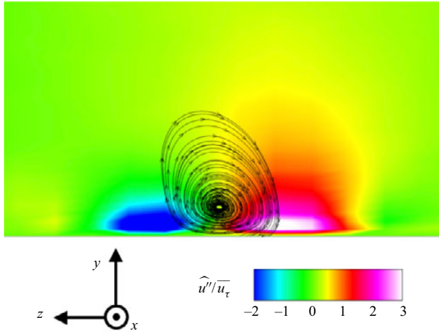
Figure 16. Cross-section streamlines computed from (\hat{v}, \hat{w}) at x = 30.0\delta_0 superimposed on the conditionally averaged streamwise velocity fluctuations obtained by the WMLES at Re_\tau \approx 2300 (same as figure 14f).
