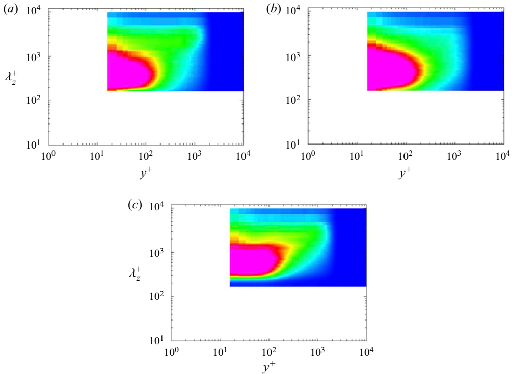
Figure 33. Premultiplied spanwise energy spectra of streamwise velocity fluctuations k_z \Phi_{u''u''} ; (a) KEEP(+filter)+SMS, (b) KEEP+SMS, (c) compact(+filter)+SMG. The colour contour is the same as that of figure 19.
