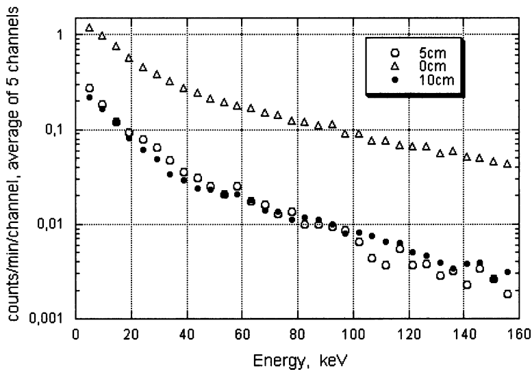
Figure 5 The LS background spectra in the underground counting room, unshielded and inside 5- and 10-cm-thick lead shields.
