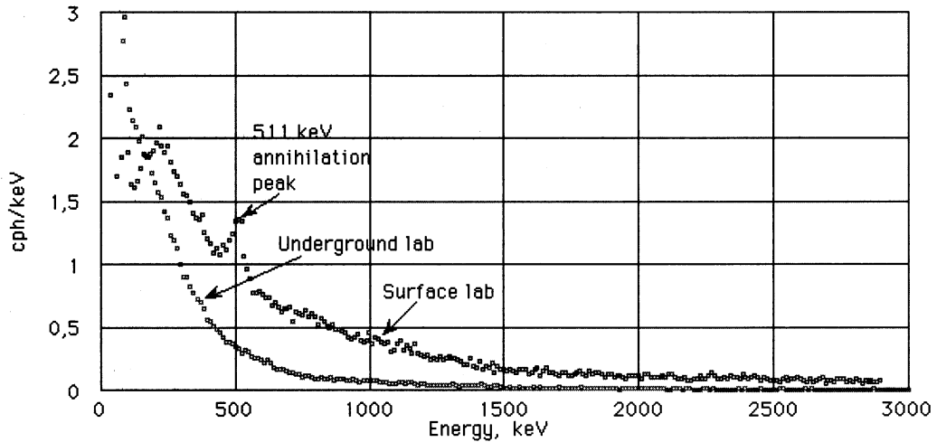
Figure 6 The NaI background spectra, with the crystal inside a 10-cm-thick shield of lead, in the surface laboratory and in the underground counting room.
