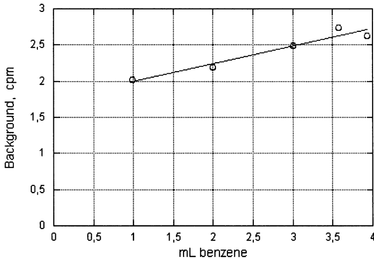
Figure 8 The LS background at varying benzene volume, measured in our surface laboratory.
