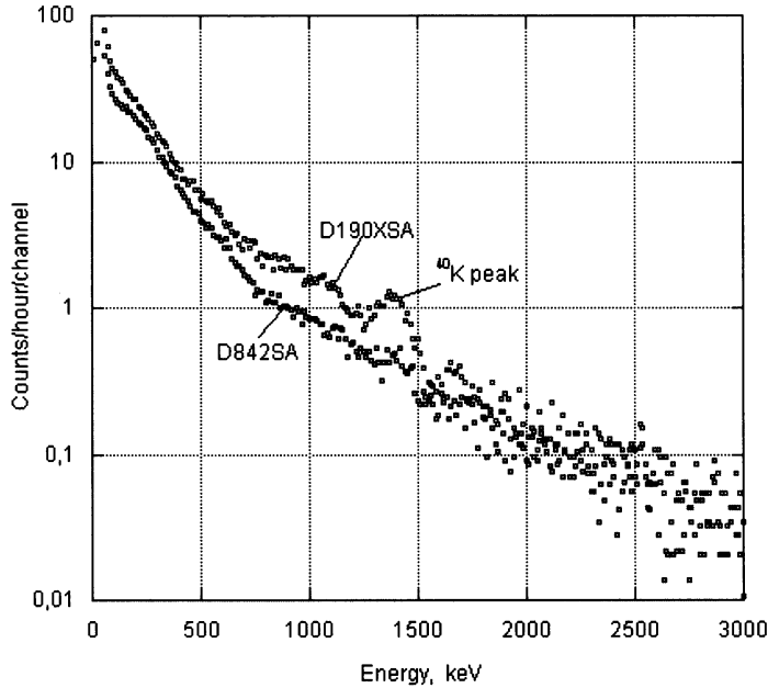
Figure 2 The background spectra with the NaI crystal on PMTs D842SA and D190XSA behind 10 cm of lead in the underground counting room. The spectra show the average values of 5 channels of a 256-channel multichannel analyzer (MCA).
