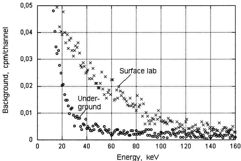
Figure 7 LS background spectra (3 mL benzene) with a 10-cm-thick lead shield in our surface laboratory and in the underground counting room.
