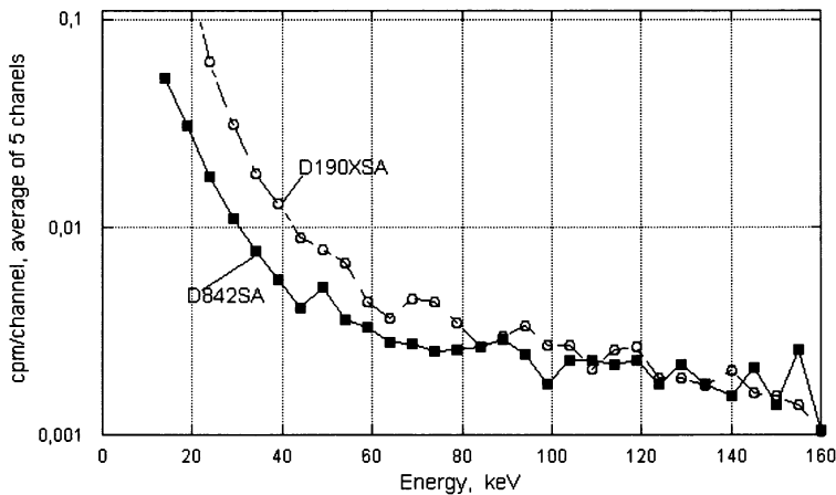
Figure 3 The LS background spectra of PMT D842SA and D190XSA behind 10 cm of lead in the underground counting room.
