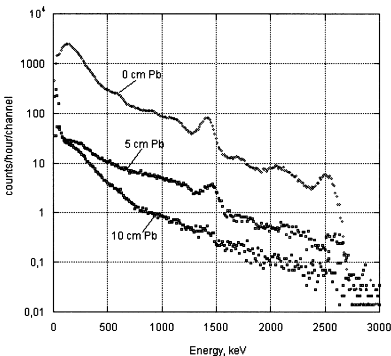
Figure 4 The NaI background spectra in the underground counting room, unshielded (0 cm) and inside 5- and 10-cm-thick lead shields.
