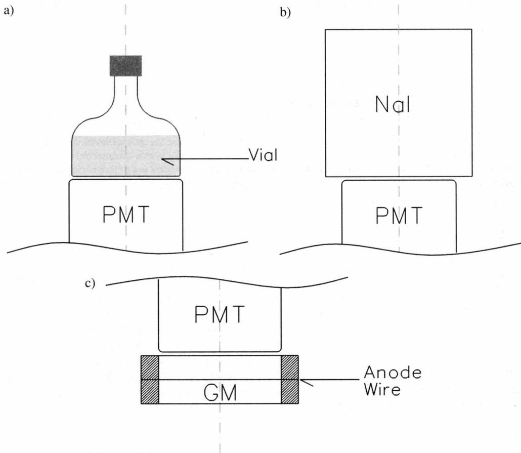
Figure 1 Detectors used in the study: a) 3-mL vial with PMT; b) NaI with PMT; c) low-level Geiger counter for measuring beta emission from the face of the PMT.
