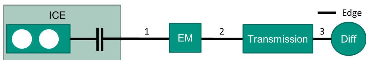
Figure 3. Schematic representation of a P2 hybrid drive train
