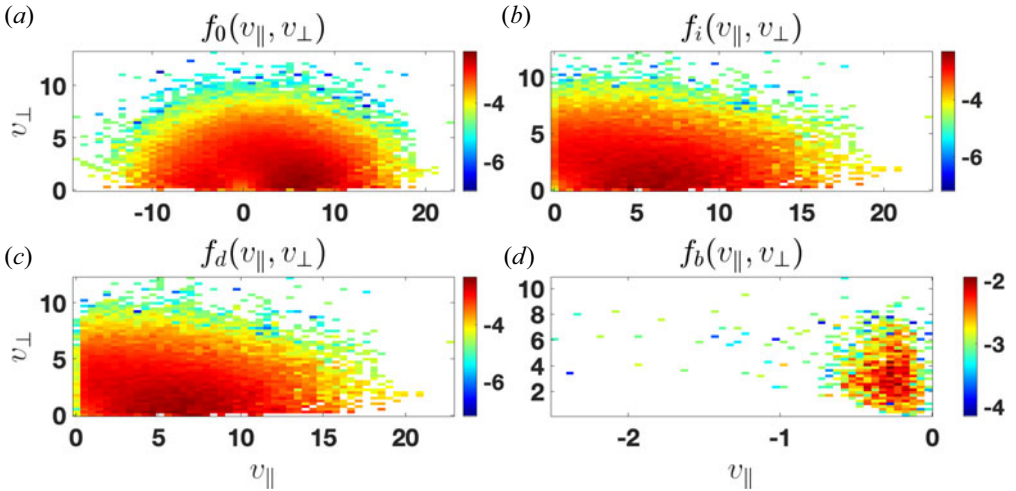
FIGURE 5. Interaction with the bipolar spike. (a) The initial bi-Maxwellian. (b) Only the incident electrons moving towards the spike. (c) The electrons crossing the spike and proceeding further downstream. (d) The backstreaming electrons reflected off the spike into the upstream region.
